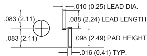
PAD/FOOTPRINT DETAIL
