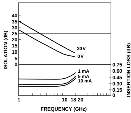
Figure 1. Typical Isolation and Insertion Loss, HPND-4028.
