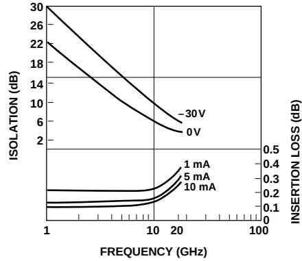
Figure 2. Typical Isolation and Insertion Loss, HPND-4038.
