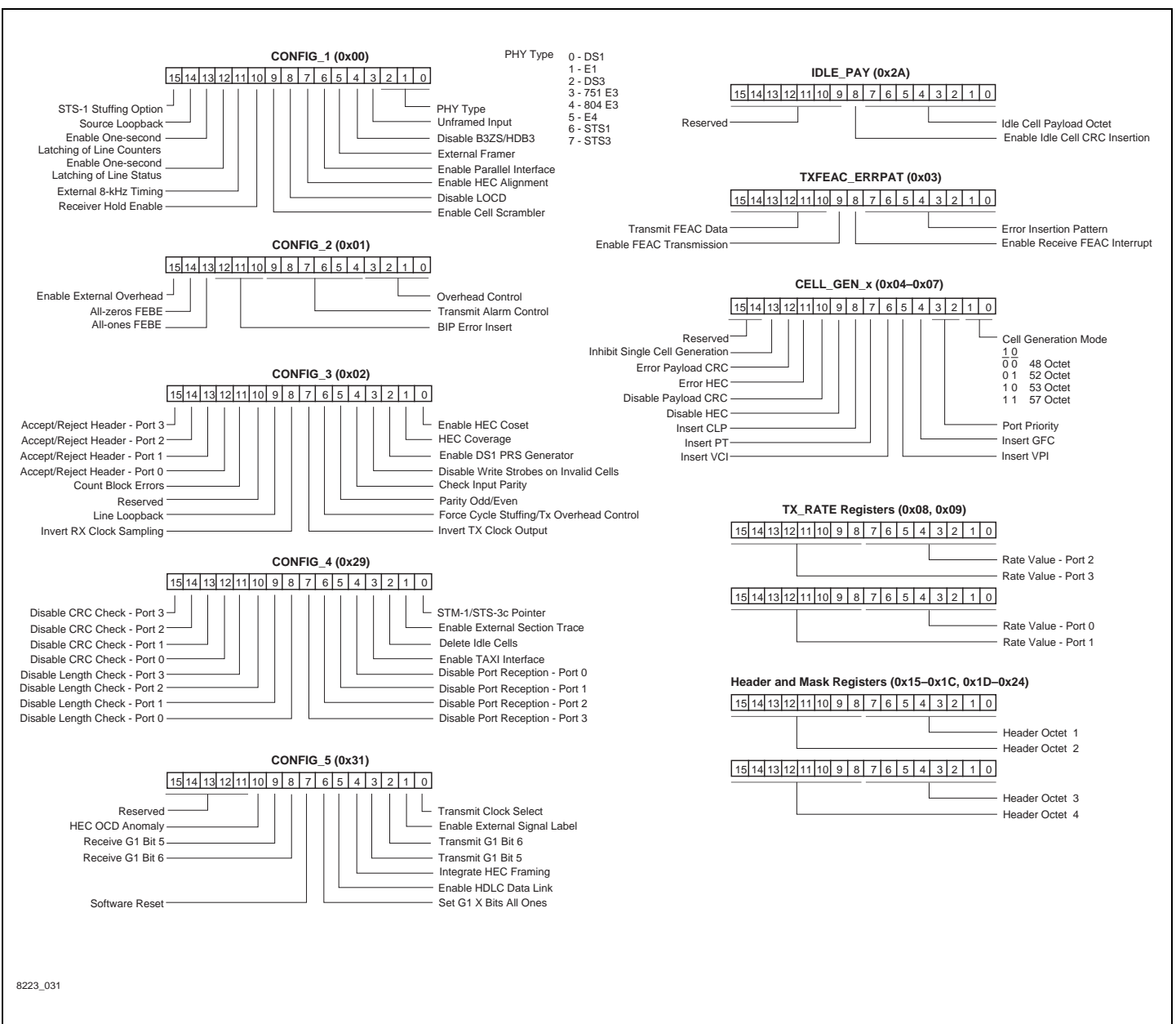
Figure 3-2. Register Summary, Cheat Sheet 1
