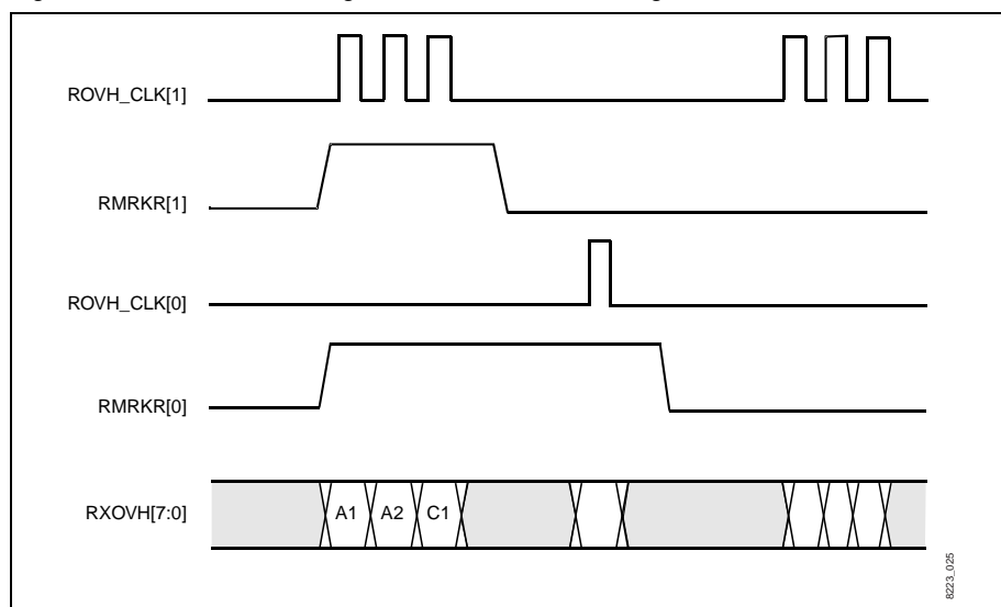
Figure 2-13. Receive Framing Overhead Interface Timing
