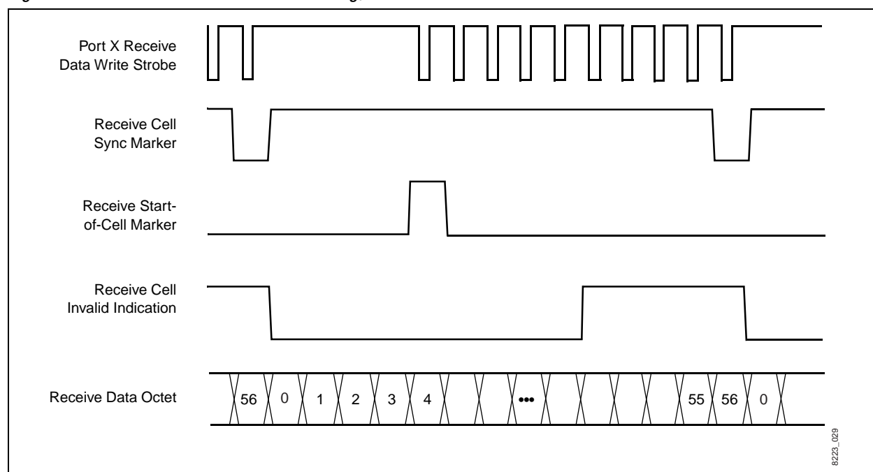
Figure 2-17. Receive FIFO Port Interface Timing, 53-Octet Mode
