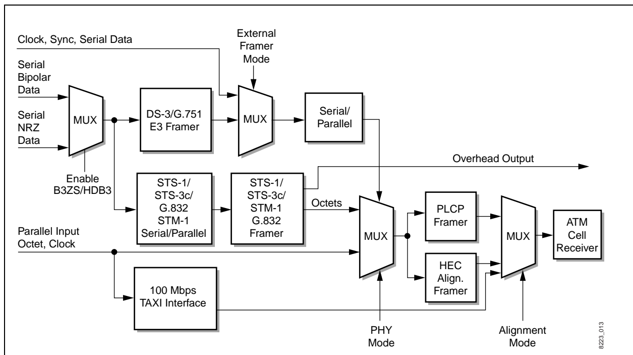
Figure 2-1. CN8223 Receiver Block Diagram
