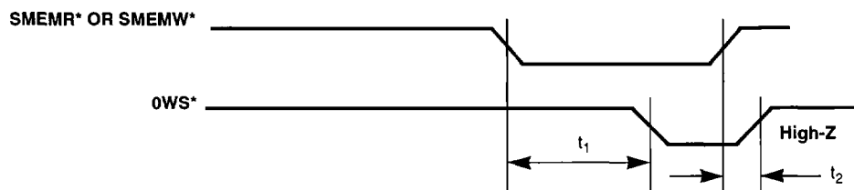
Figure 7-9. OWS* Timing (ISA Bus)
