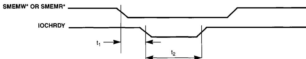
Figure 7-8. IOCHRDY for Memory Access Timing (ISA Bus)
