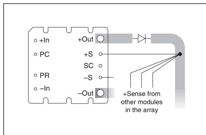
Figure 12 — OR'ing diodes connections.
