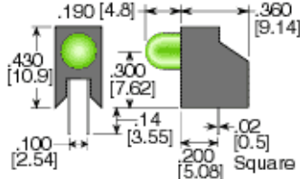
Series PCT230 Figure 1. Standard Projection
