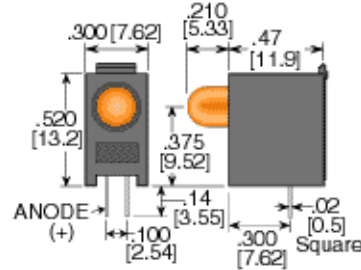
Series PCT240 Figure 2. Low Projection
