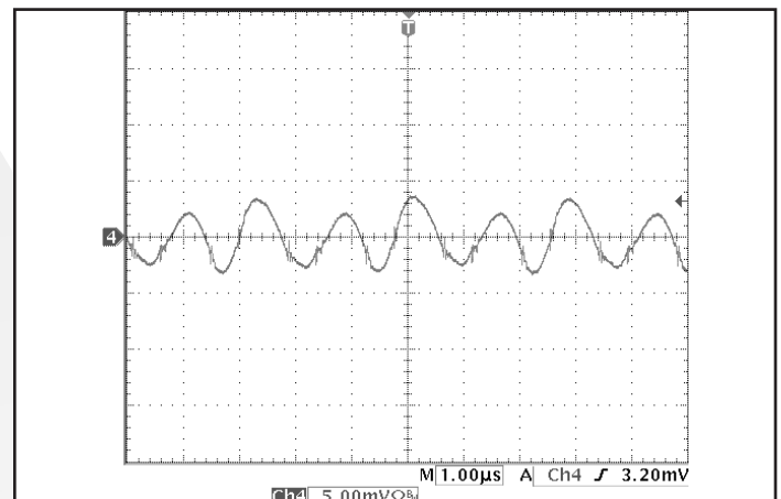
Figure 10: Output voltage ripple, Vout, at nominal input voltage and rated load current (5 mV/div). Load capacitance: 1µF ceramic capacitor and 10µF tantalum capacitor. Bandwidth: 10 MHz. See Figure 17.
