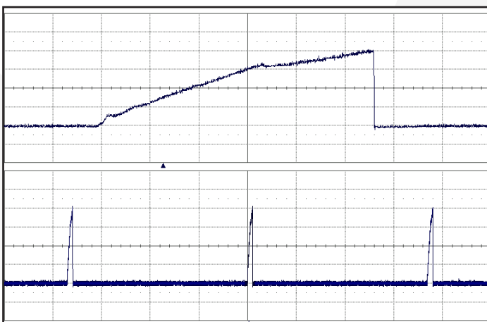
Figure 5: Load current (5A/div) as a function of time (2ms/div and 100ms/div) when the converter attempts to turn on into a 10 mΩ short circuit.
