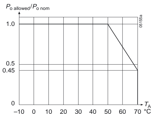
Fig. 4 Maximum allowed output power versus ambient temperature at V_i > 105 \text{ VAC} for LOK models.
