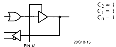
Figure 8. Pin 13 OE/Active HIGH
