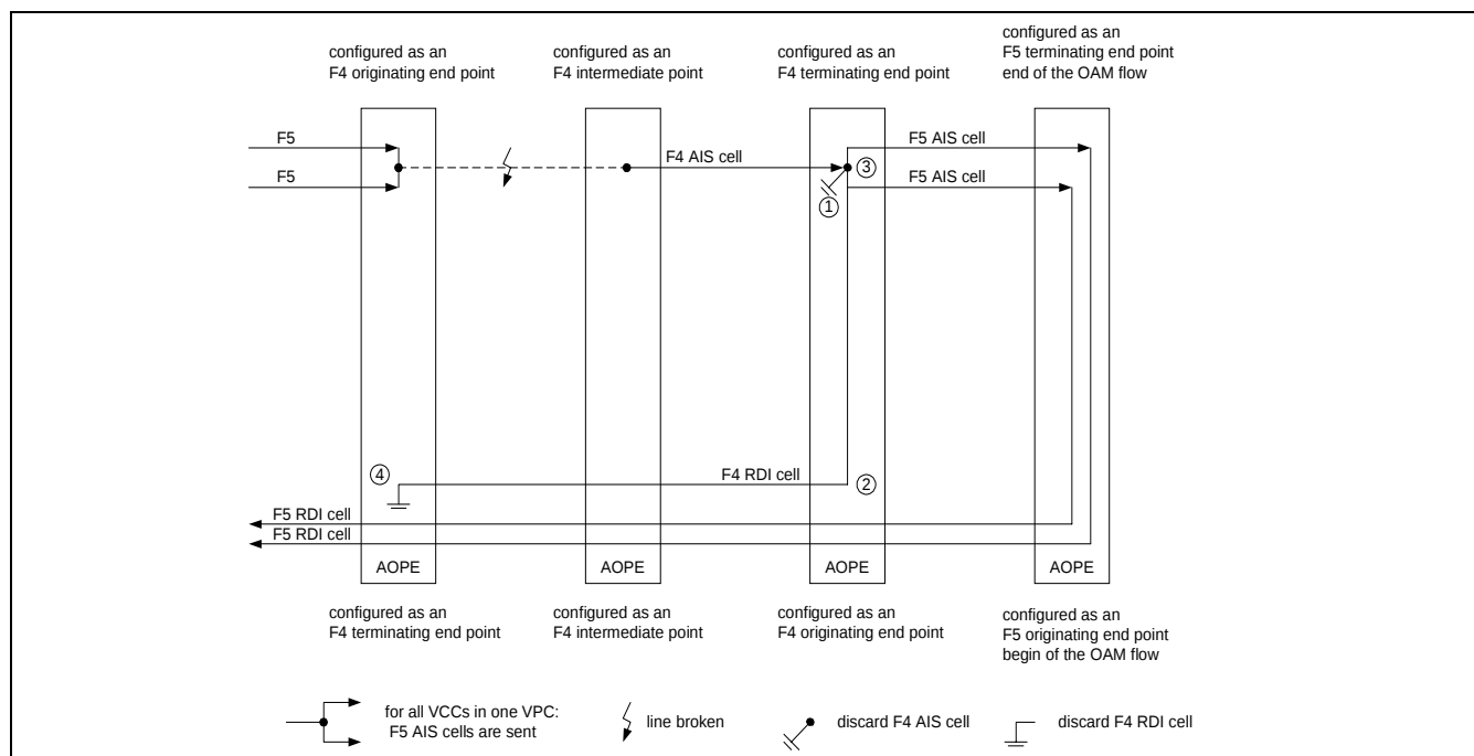
Figure 16 VP-AIS/RDI-Flow (F4-AIS/RDI-Flow)
