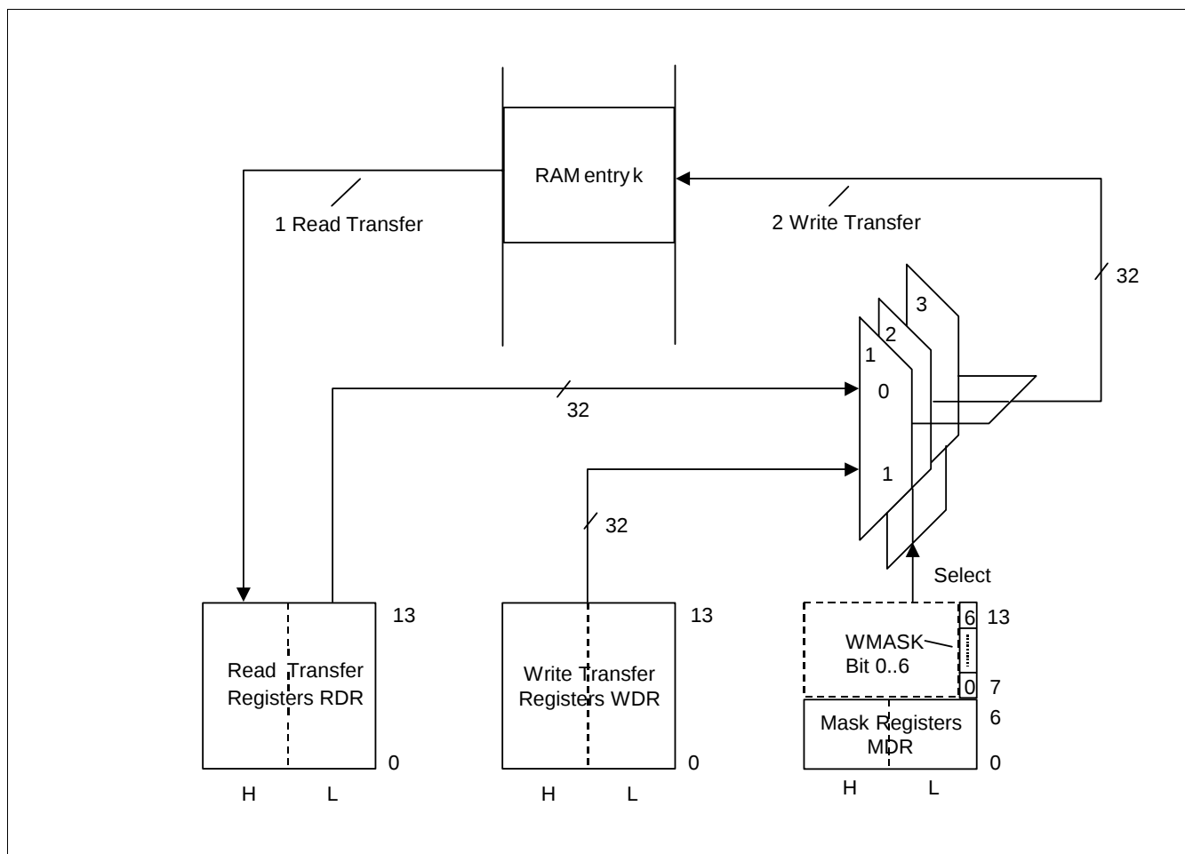
Figure 32 Read-modify-write Transfer
