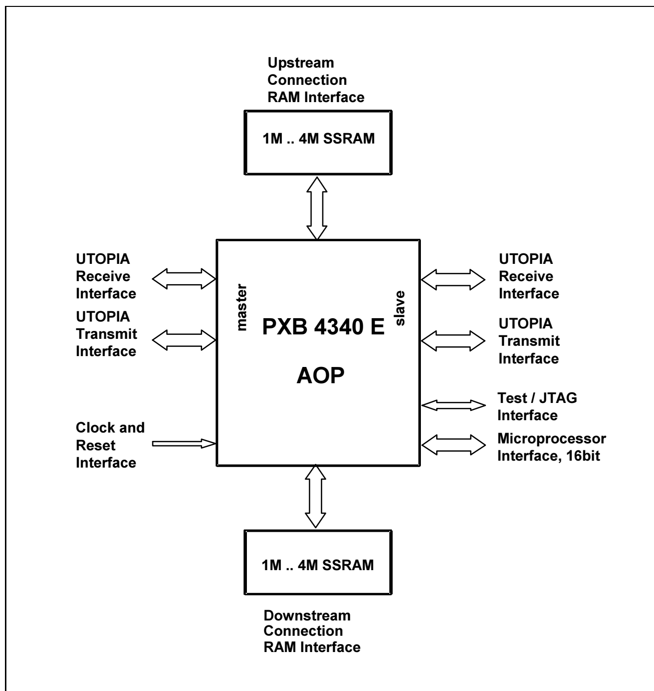
Figure 6 Logic Symbol
