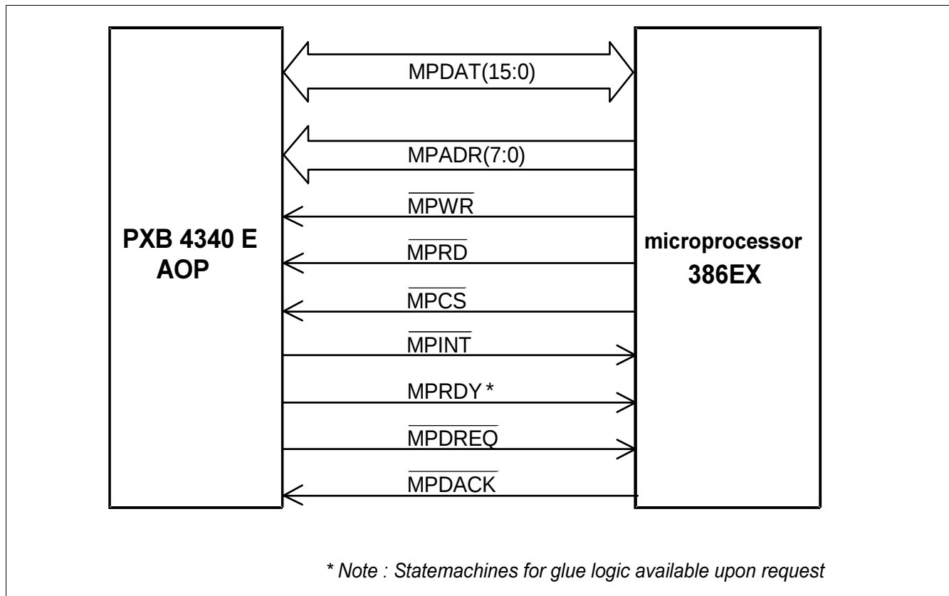
Figure 41 Microprocessor Interface
