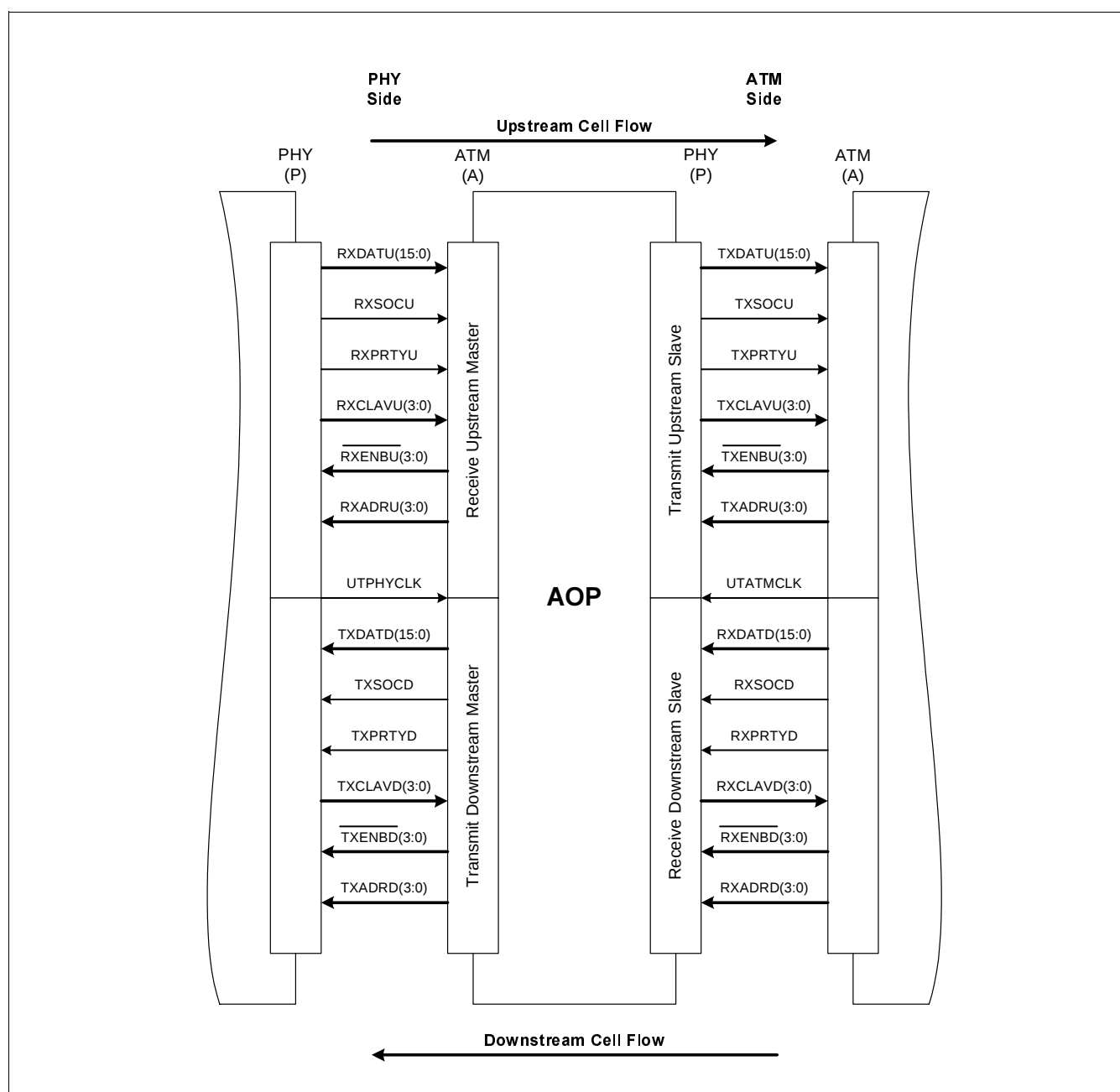
Figure 34 UTOPIA Interfaces
