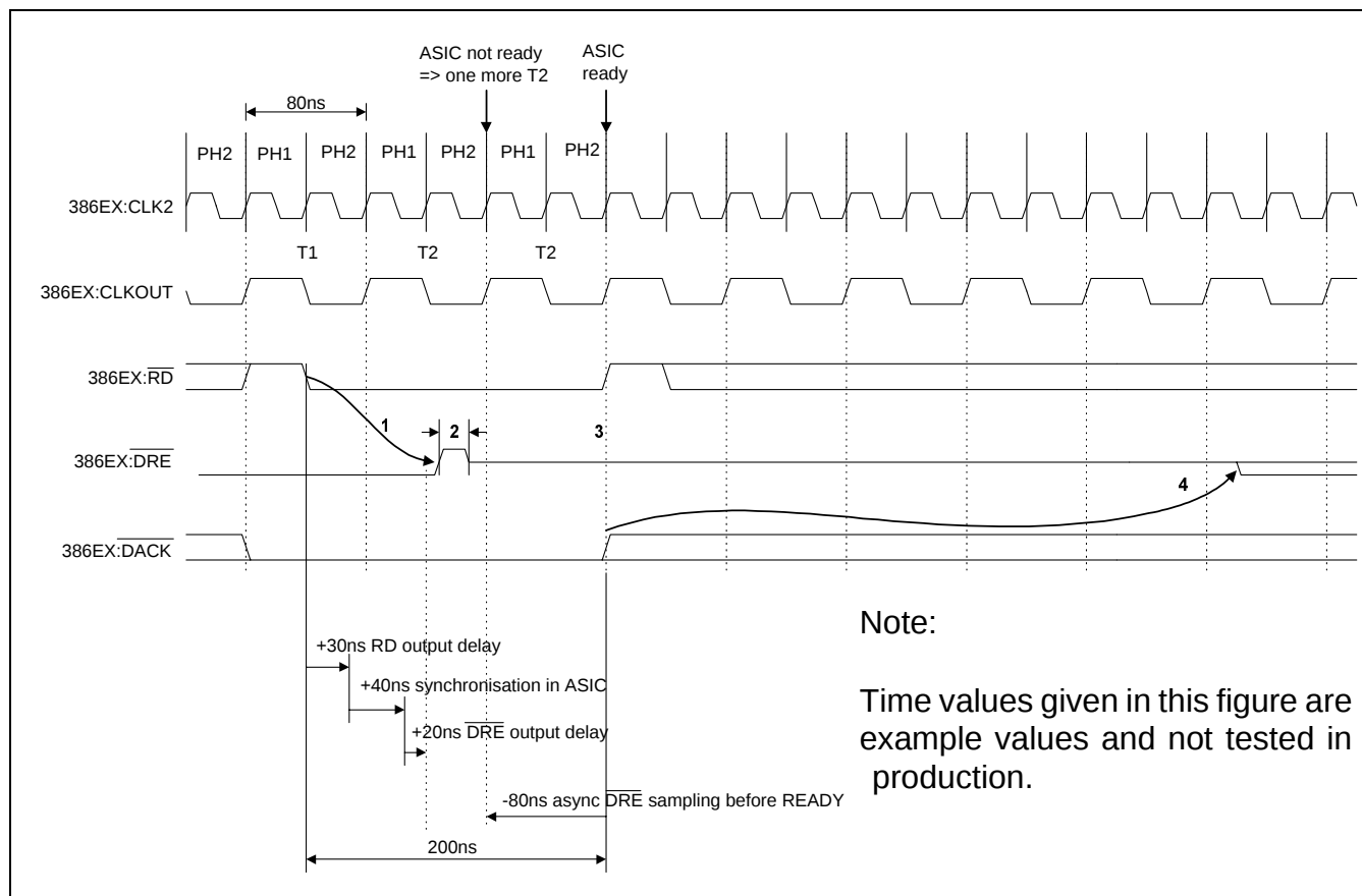
Figure 46 Microprocessor DMA Interface
