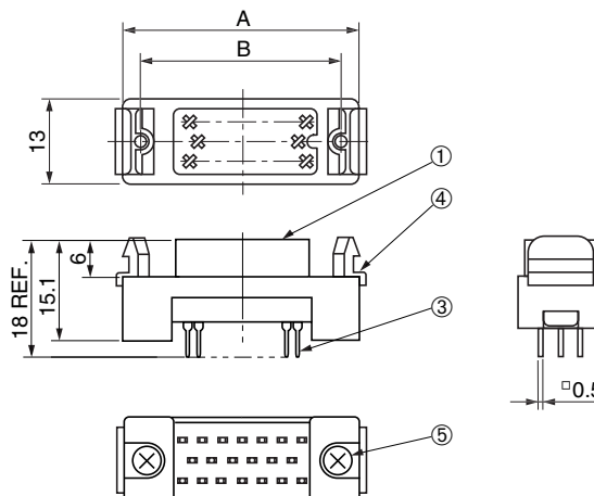
16, 20, 25, 34 or 50-contact connector
