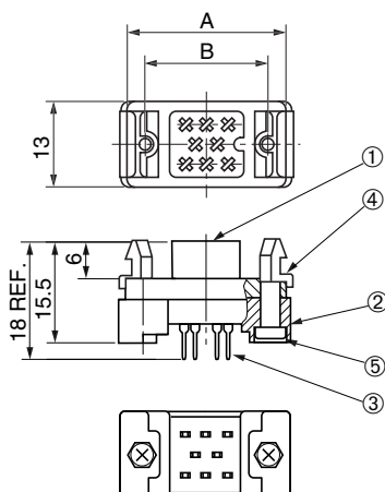
8-contact connector
