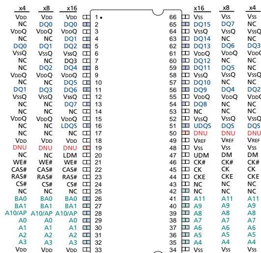
Figure 1: Pin Assignment (Top View) 66-pin TSOP
