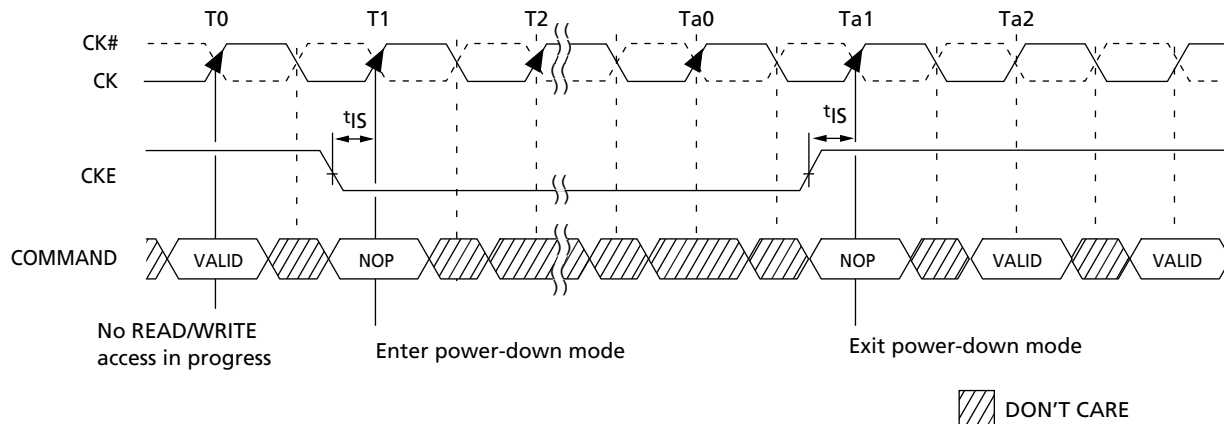
Figure 32: Power-Down
