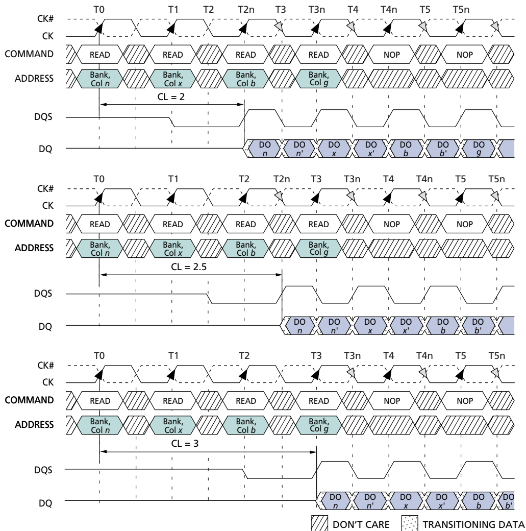
Figure 16: Random READ Accesses
