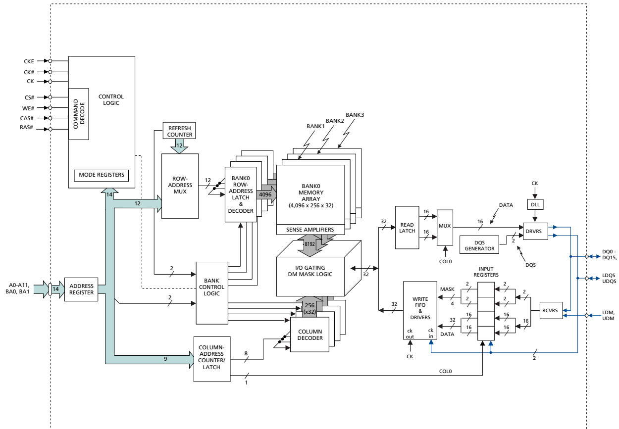
Figure 5: Functional Block Diagram 8 Meg x 16
