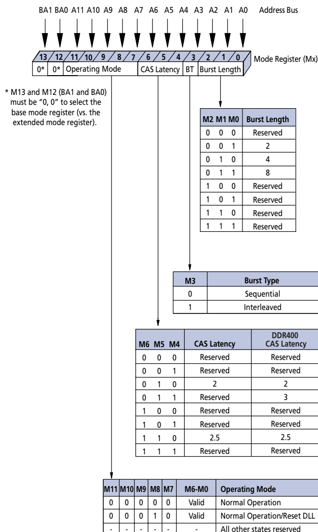
Figure 7: Mode Register Definition
