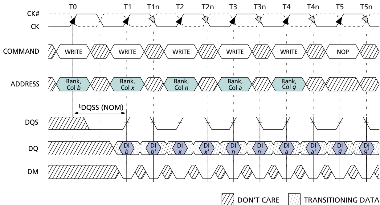
Figure 24: Random WRITE Cycles
