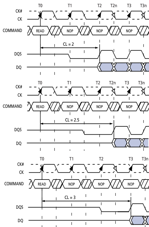
Figure 8: CAS Latency
