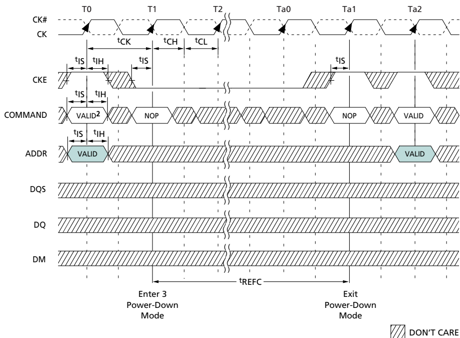
Figure 46: Power-Down Mode
