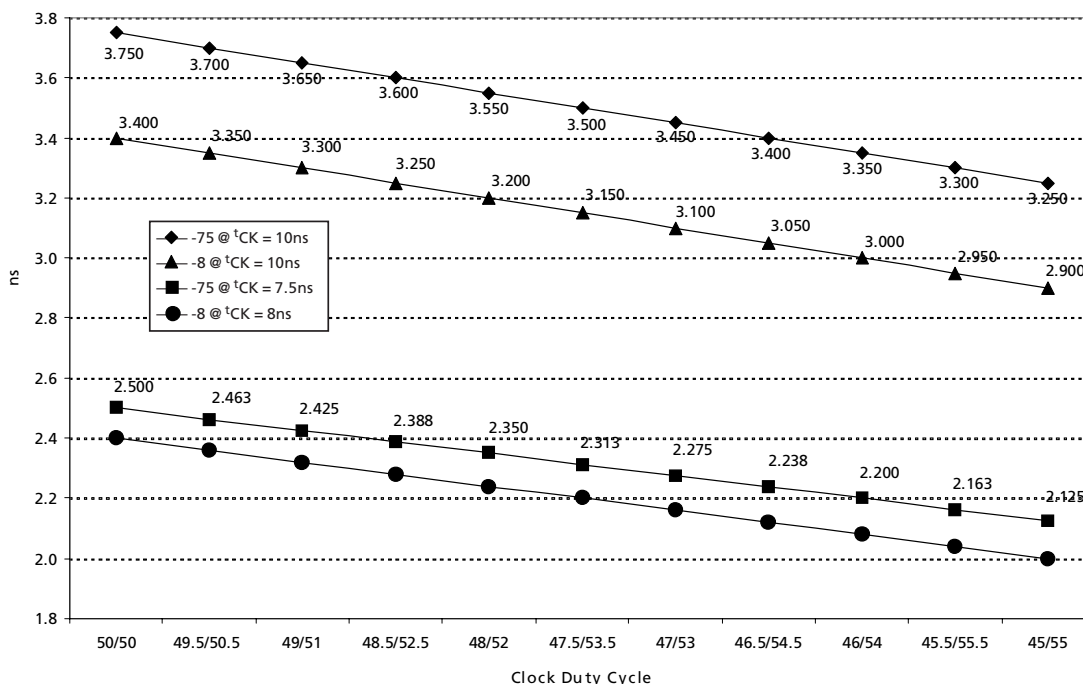
Figure 35: Derating Data Valid Window ( t_{QH} - t_{DQSQ} )
