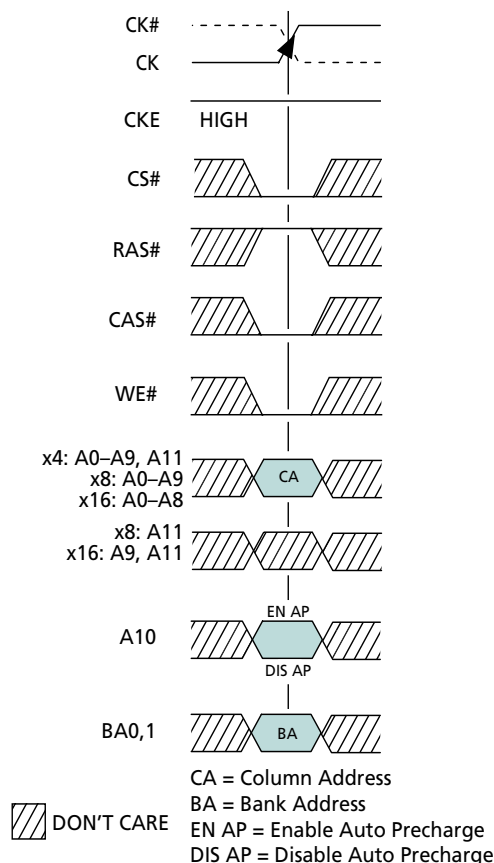
Figure 20: WRITE Command
