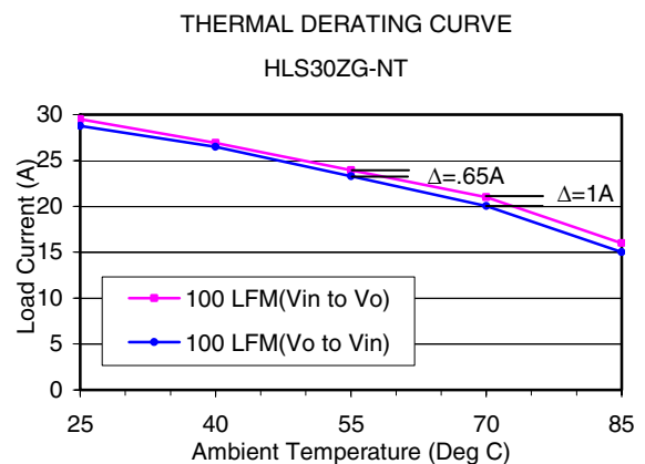
Figure 15. HLS30ZD (2.5V) Derating
