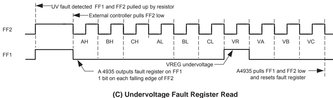
Figure 1. Fault flag sequence diagrams
