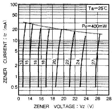
Fig. 2 RLZ13 ~ RLZ27 Zener characteristic
