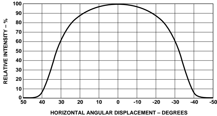
Figure 8. Spatial radiation pattern – 35 x 70 degree lamps.
