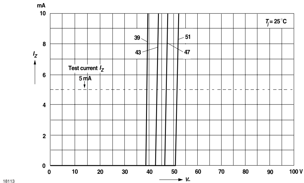
Figure 14. Breakdown Characteristics
