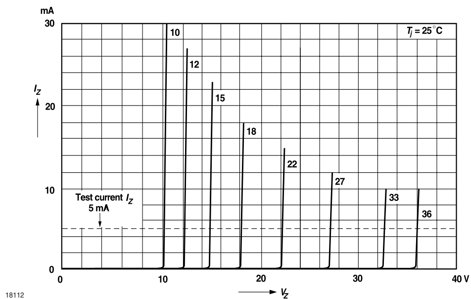
Figure 13. Breakdown Characteristics
