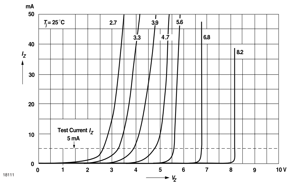
Figure 12. Breakdown Characteristics
