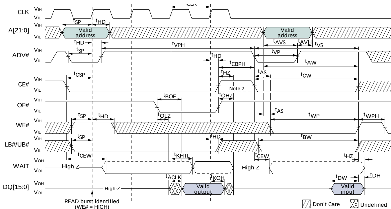
Figure 53: Burst READ Followed by Asynchronous WRITE Using ADV#
