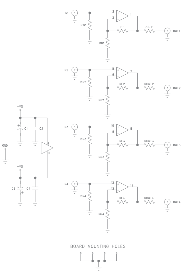
Figure 10. CEB018 Schematic
