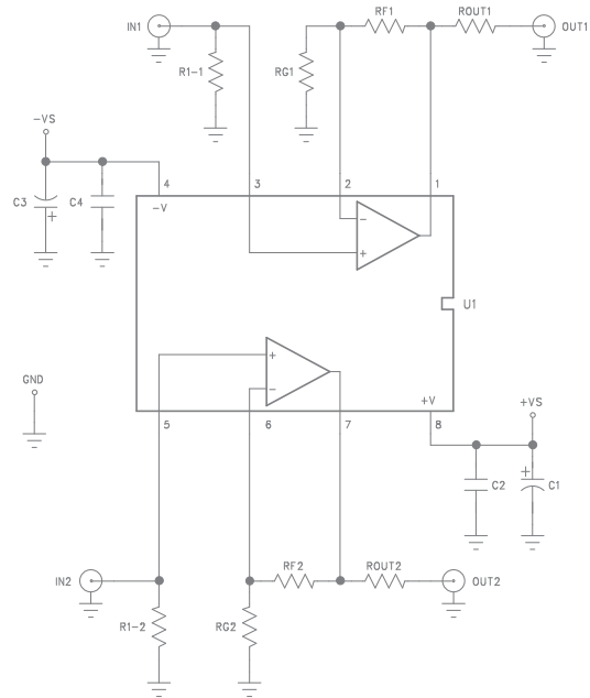
Figure 7. CEB006 Schematic
