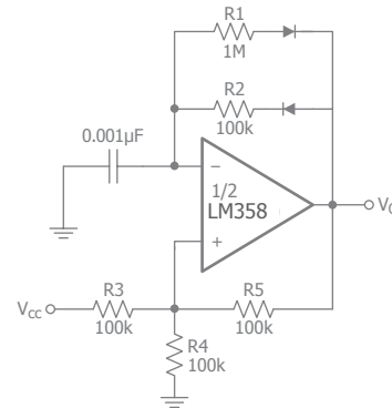
Figure 18. Pulse Generator
