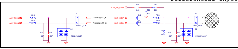
Differential Input
