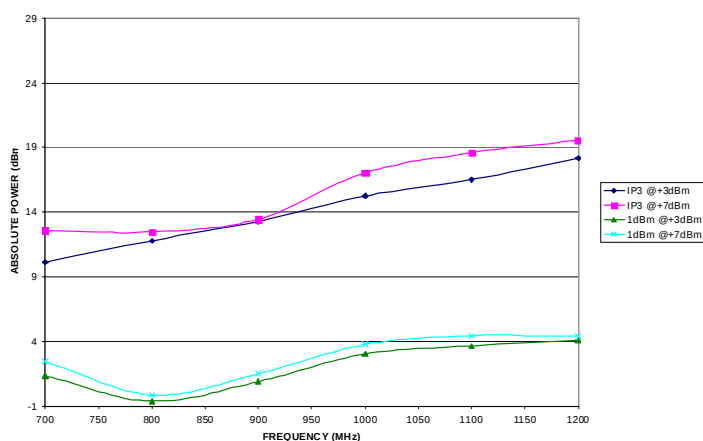
Third Order Intercept and Input 1 dB Compression Power
