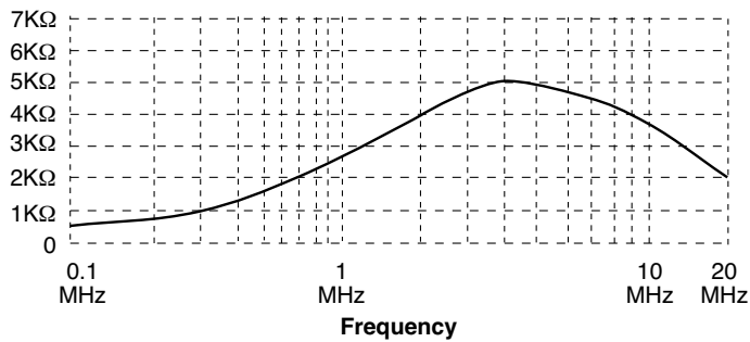
Impedance Curve
