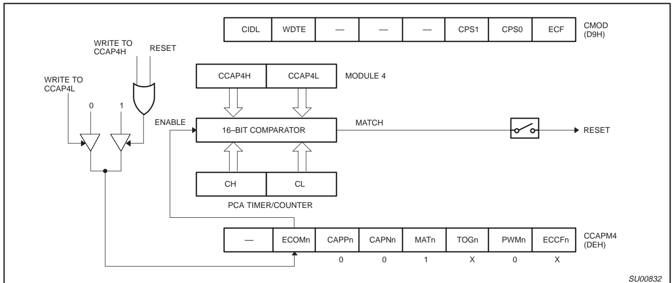
Figure 25. PCA Watchdog Timer m(Module 4 only)
