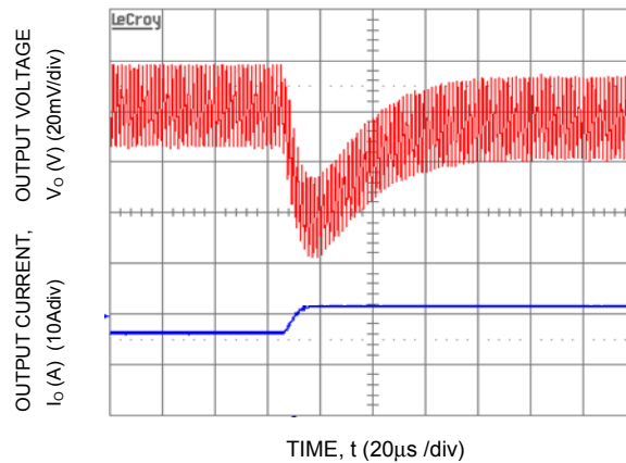
Figure 22. Transient Response to Dynamic Load Change from 50% to 100% at 12Vin, C_{out}=1 \times 47\mu\text{F} + 1 \times 330\mu\text{F} , C_{Tune}=3300\text{pF} & R_{Tune}=270\text{ohms}
