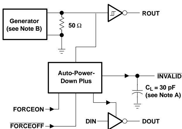
TEST CIRCUIT
