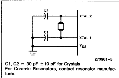
Figure 4. Oscillator Connections
