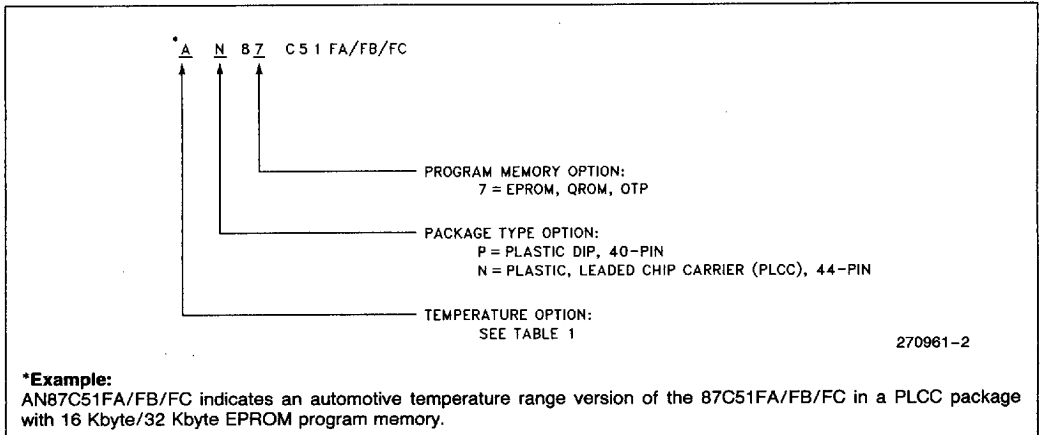
Figure 2. Package Options
