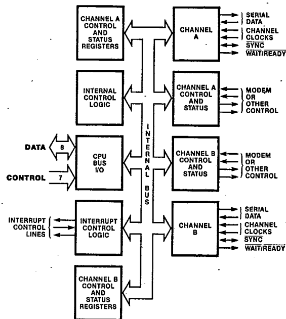
Figure 8. Block Diagram
