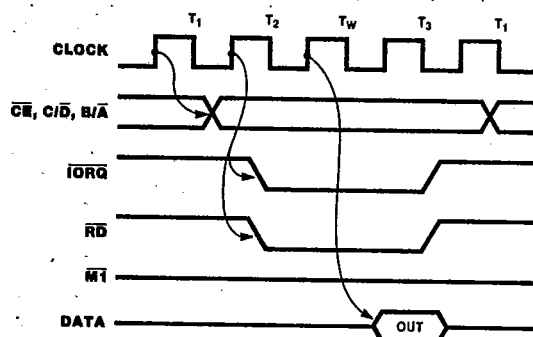
Figure 15. Read Cycle
