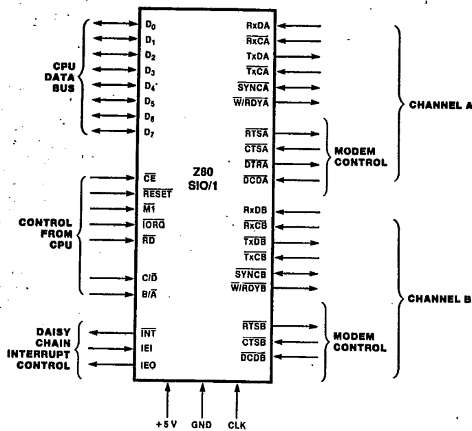
Figure 3. Pin Functions
