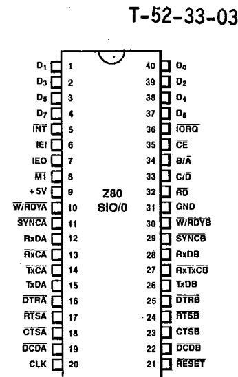
Figure 6. 40-pin Dual-In-Line Package (DIP), Pin Assignments
