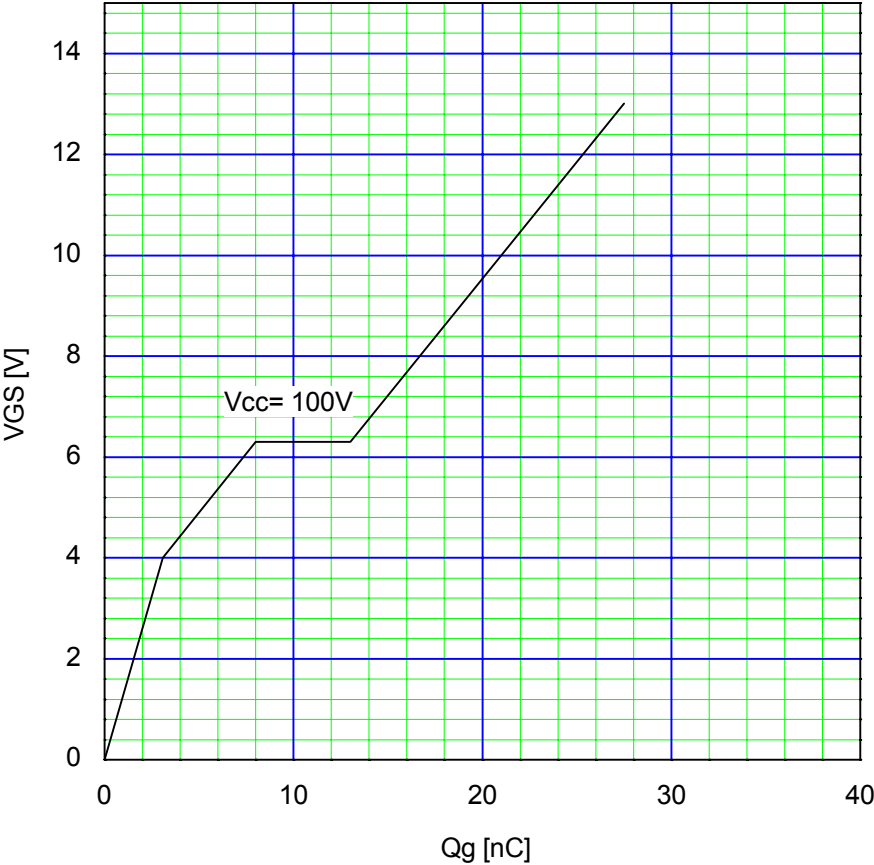
Typical Gate Charge Characteristics V GS =f(Q g ):I D =13A,T ch =25°C
