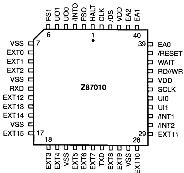
Figure 2. 44-Pin PLCC Pin Assignments
