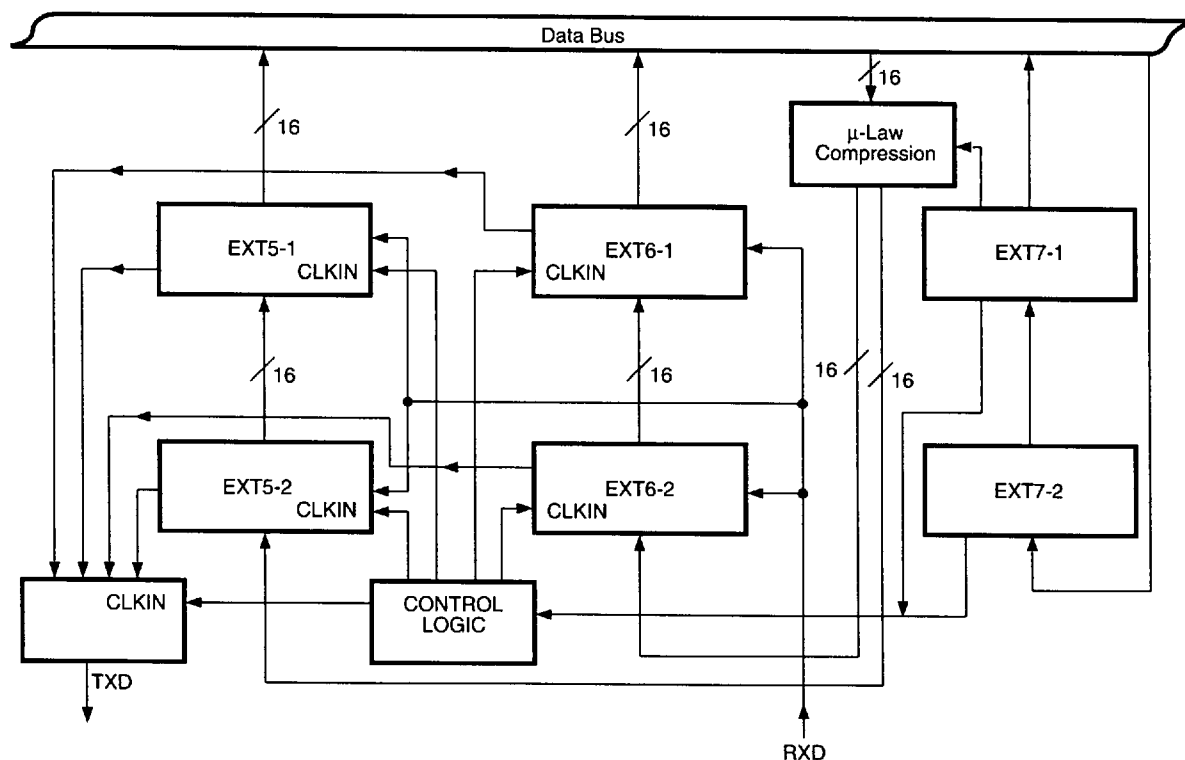
Figure 9. CODEC Interface Block Diagram
