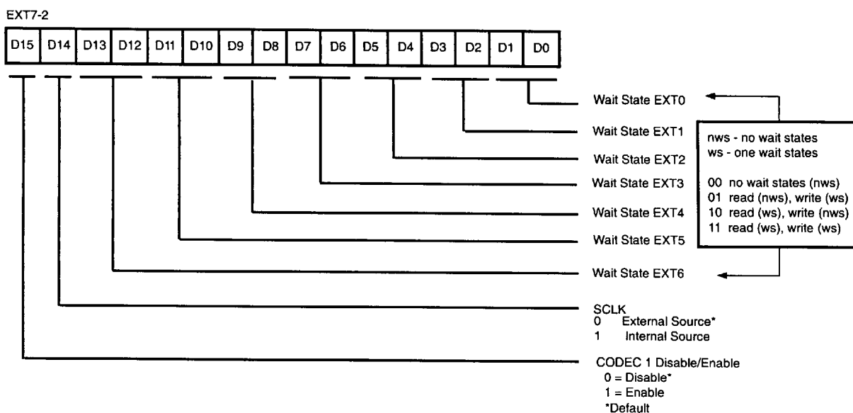
Figure 14. Wait/State/CODEC Interface Control Register
