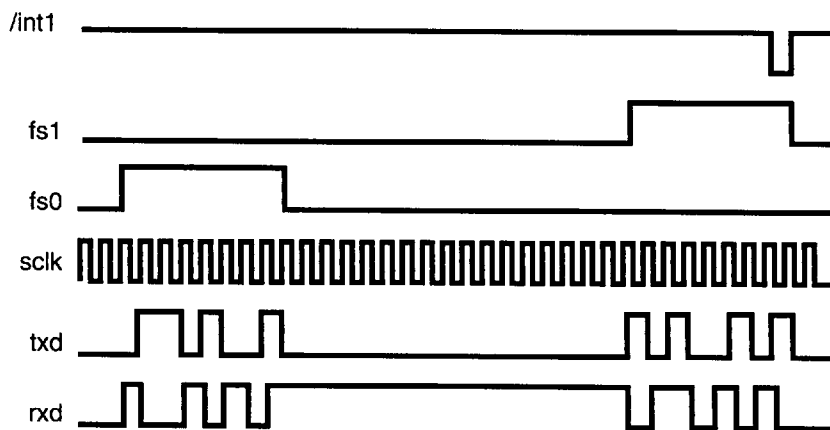
Figure 10. CODEC Interface Timing (8-Bit Mode)
