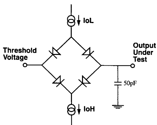
Figure 4. Test Load Diagram
