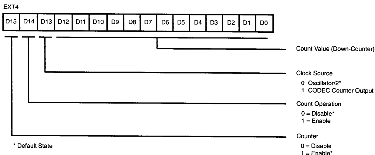
Figure 15. Timer Register
