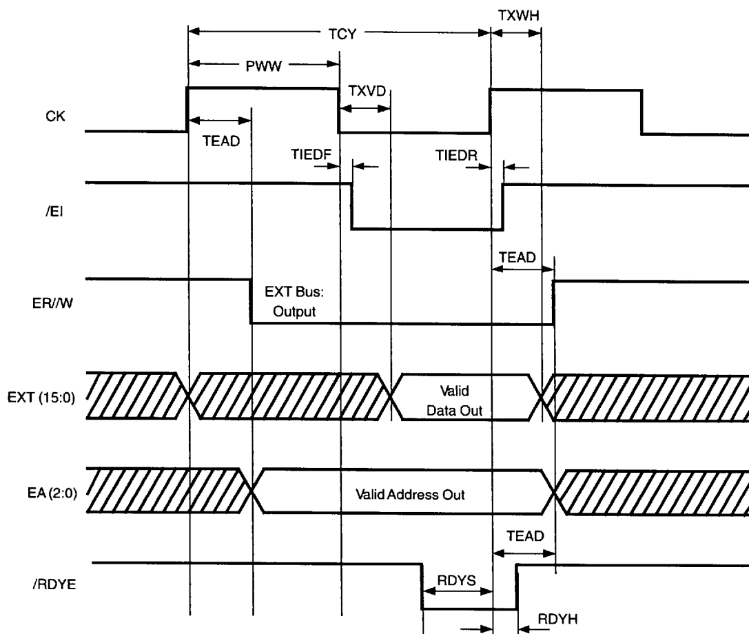
Figure 5. Write to External Device Timing
