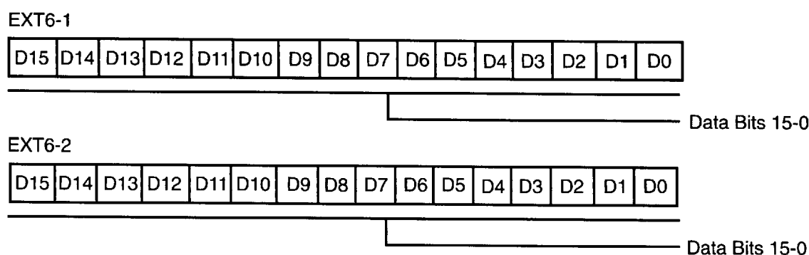
Figure 12. CODEC Interface Data Registers (Channel 1)
