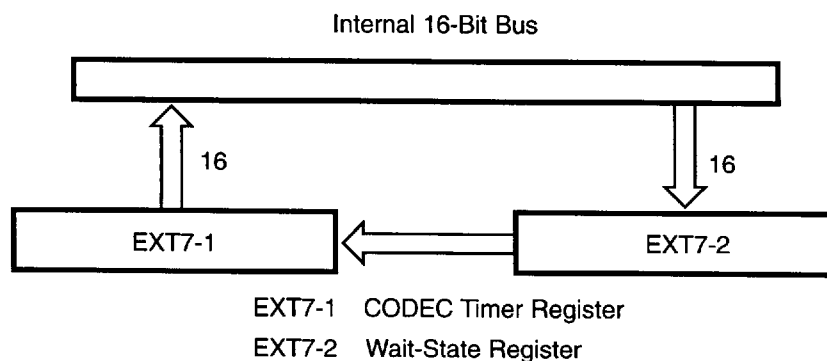
Figure 16. EXT7 Register Configuration
