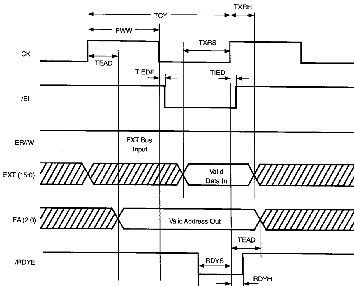
Figure 6. Read From External Device Timing
