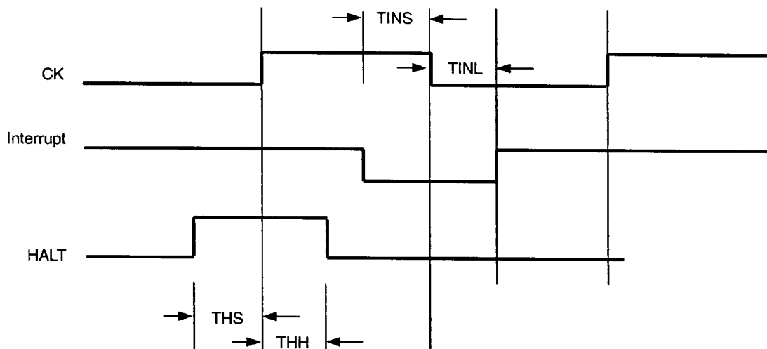
Figure 7. Interrupt/HALT Timing
