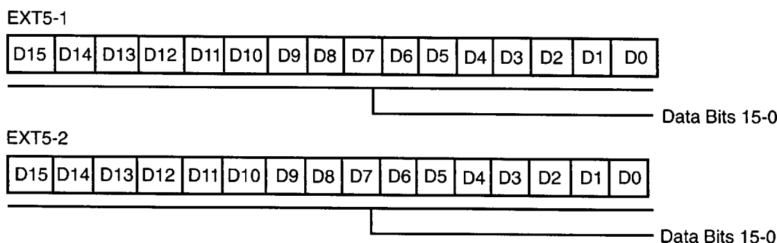
Figure 11. CODEC Interface Data Registers (Channel 0)
