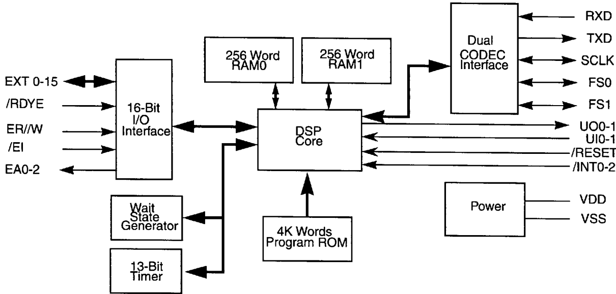
Figure 1. Z87010 Functional Block Diagram
