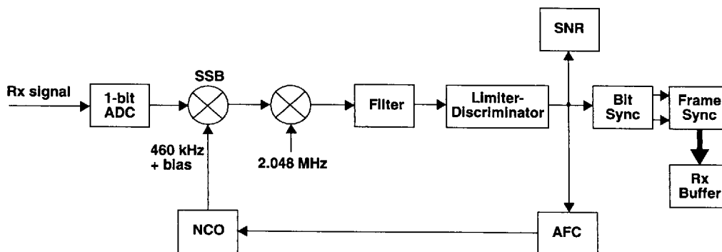
Figure 2. Demodulator Block Diagram
