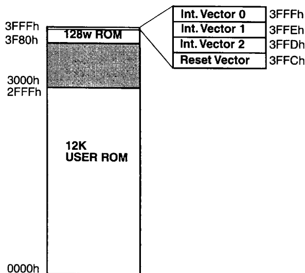
Figure 4. ROM Mapping
