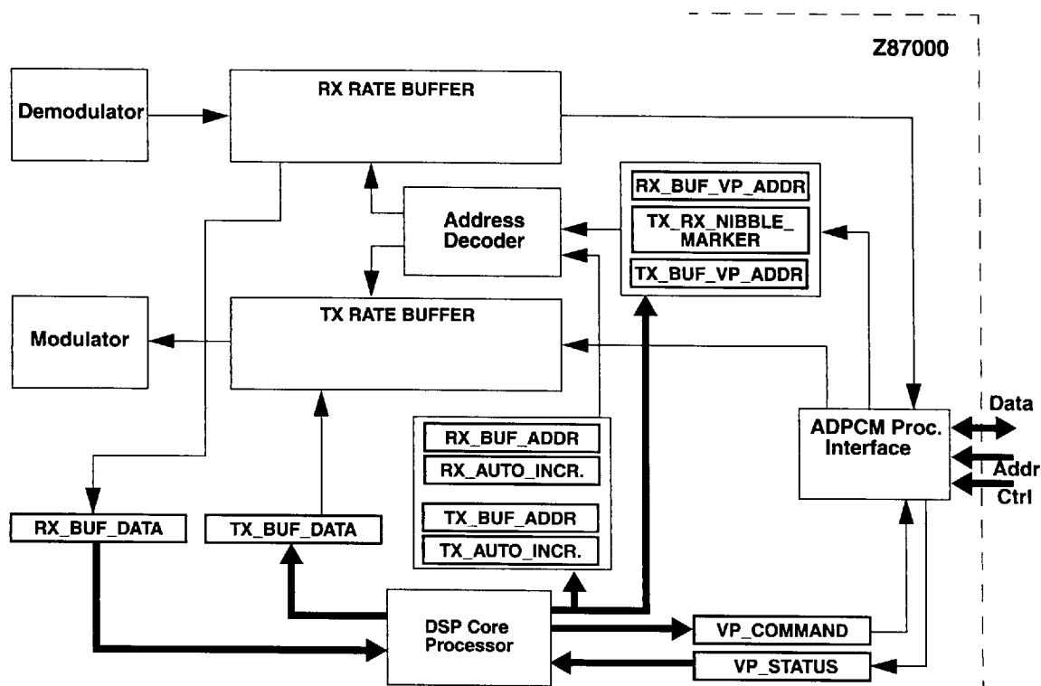
Figure 9. Rate Buffers Access and ADPCM Processor Interface
