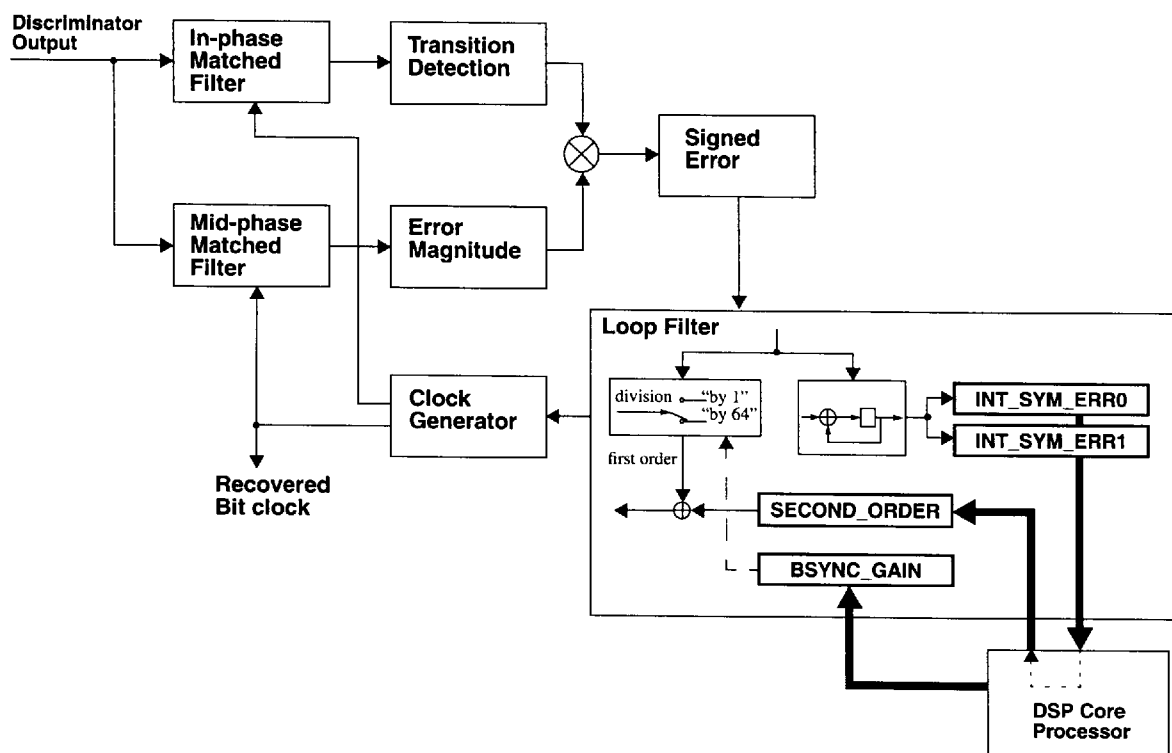
Figure 6. Bit Synchronizer Loop and Processor Control
