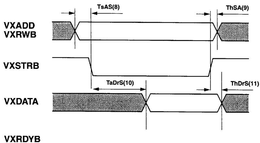
VXDATA Read Cycle
