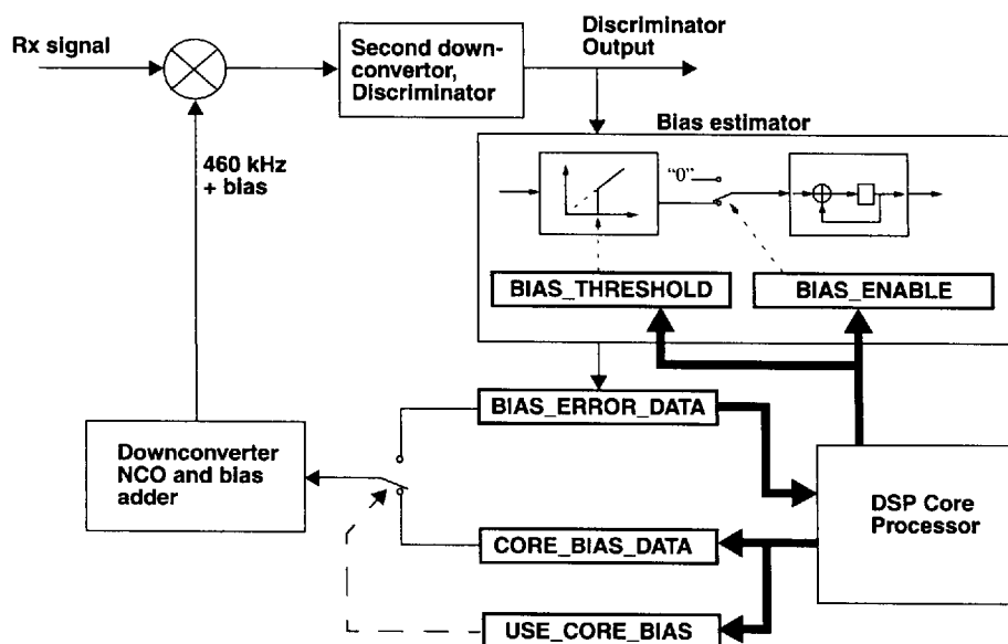
Figure 5. AFC Loop and Processor Control
