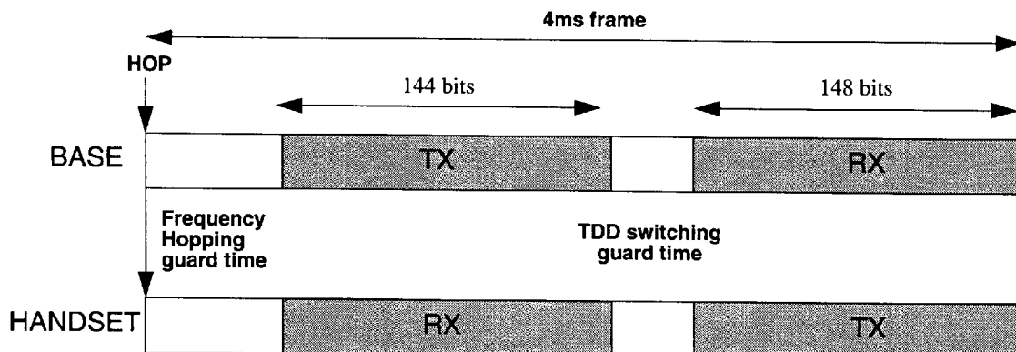
Figure 1. Basic Time Duplex Timing
