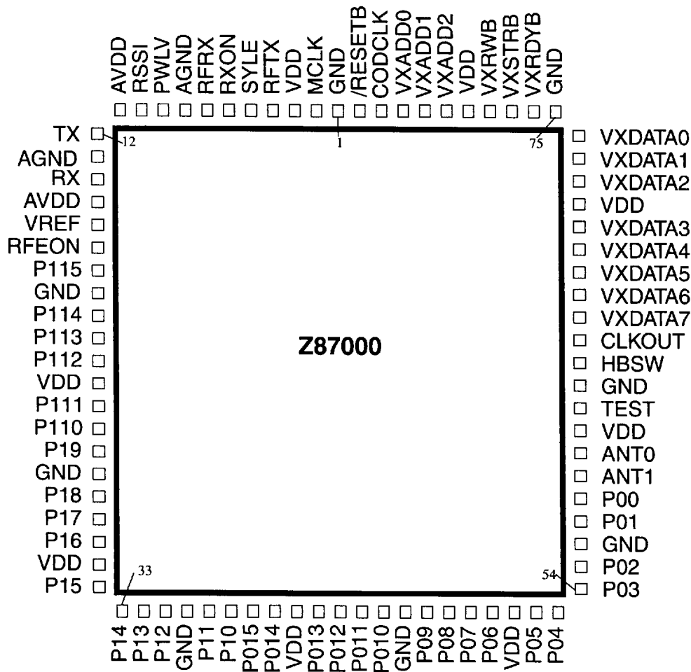
Figure 3. 84-Pin PLCC ROM Pin Configuration (Z87000 only)
