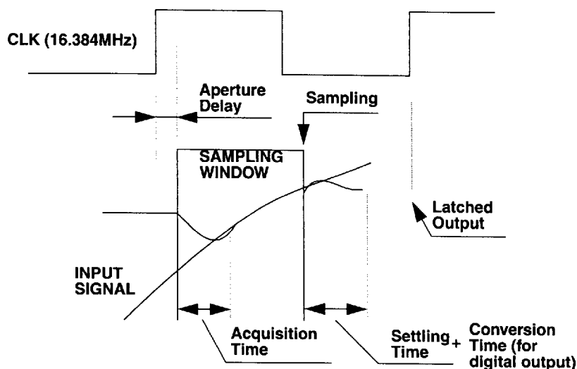
Figure 6. 1-Bit ADC Definition of Terms
