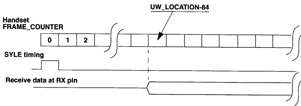
Figure 7. Frame Counter and UW_LOCATION on Handset
