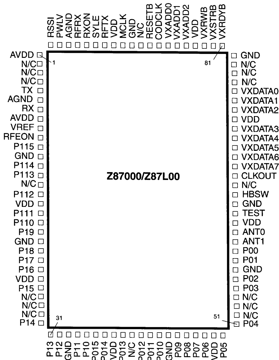
Figure 4. 100-Pin QFP Pin Configuration
