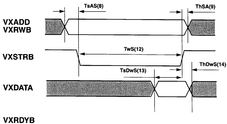
VXDATA Write Cycle
