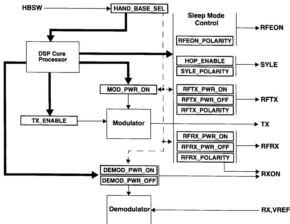
Figure 8. RF interface Control
