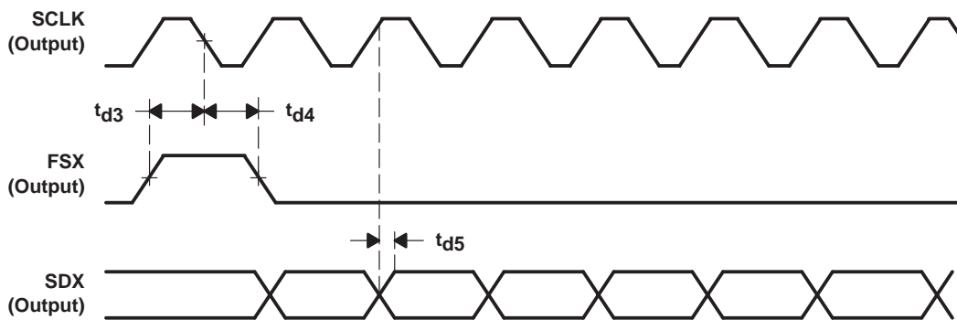
Figure 11. Data Transfers From TLFD500PN to DSP
