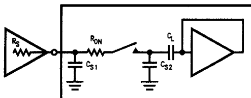
FIGURE 5. Analog Input Model
