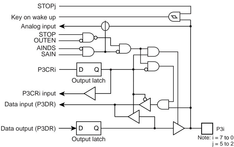
Figure 7-5 Port P3
