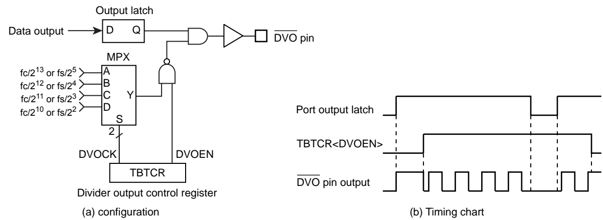
Figure 5-3 Divider Output
