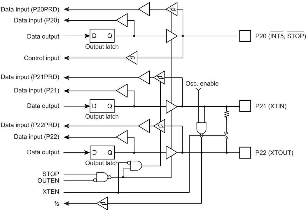
Figure 7-4 Port P2
