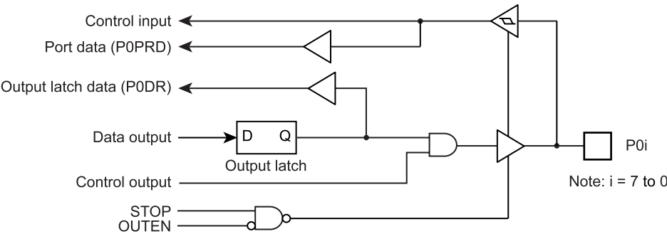
Figure 7-2 Port P0
