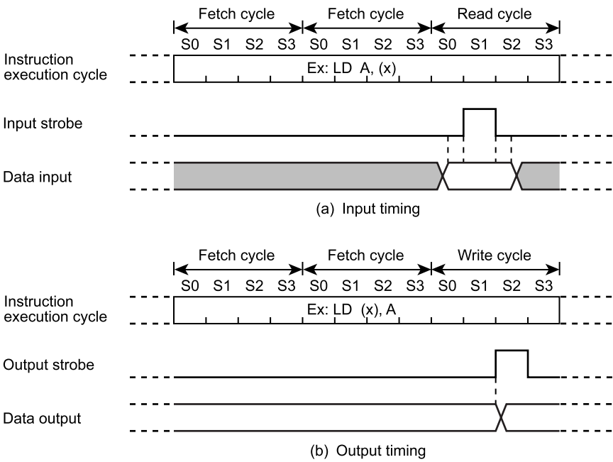
Figure 7-1 Input/Output Timing (Example)
