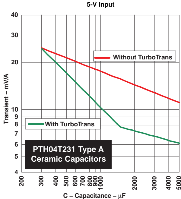
Figure 10. Capacitor Type A, 100 < C(\mu F) \times ESR(m\Omega) \leq 1000 (e.g. Ceramic)
