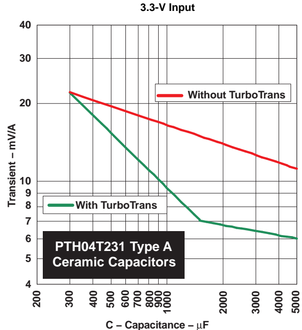
Figure 11. Capacitor Type A, 100 < C(\mu F) \times ESR(m\Omega) \leq 1000 (e.g. Ceramic)
