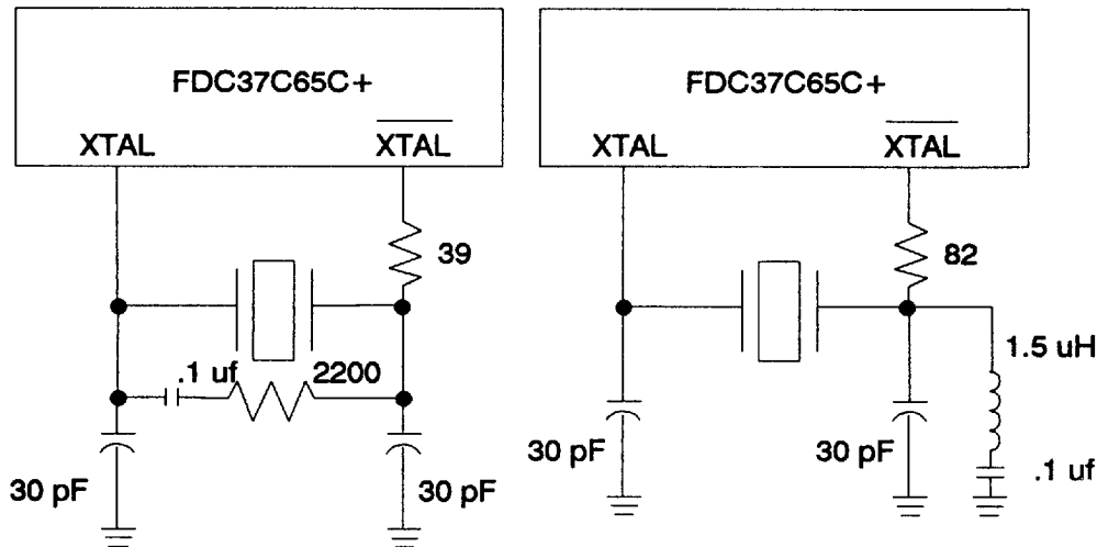
FIGURE 2 - SUGGESTED OSCILLATOR CIRCUITS
