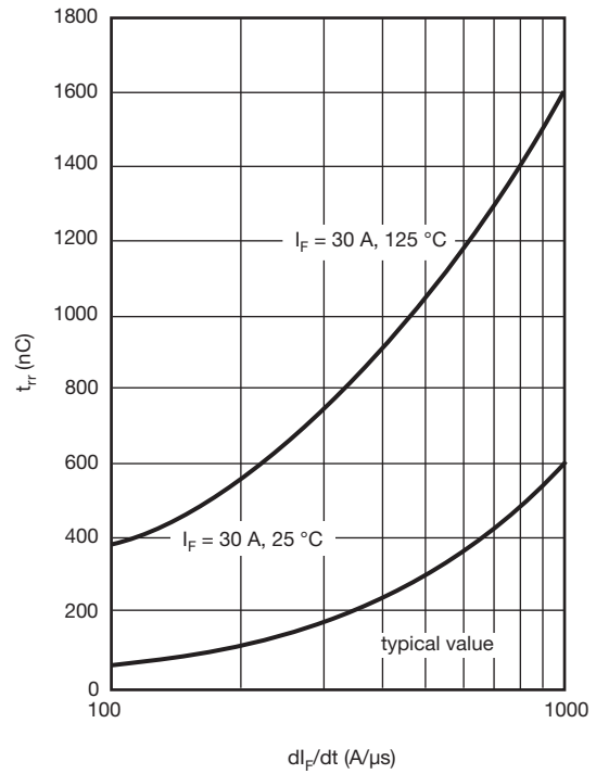
Fig. 8 - Typical Stored Charge vs. di/dt
