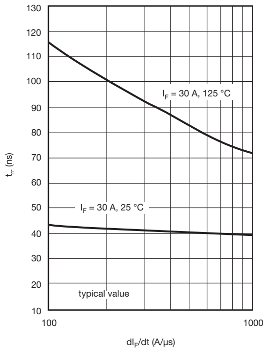
Fig. 7 - Typical Reverse Recovery vs. di/dt
