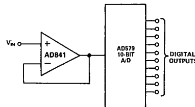
Figure 8. Input Buffer
