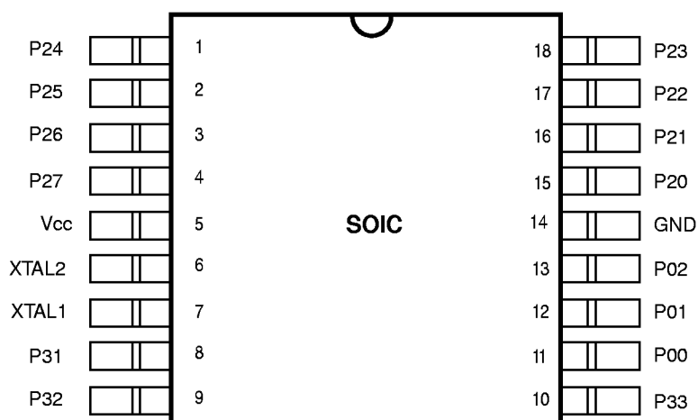
Figure 3. 18-Pin SOIC
