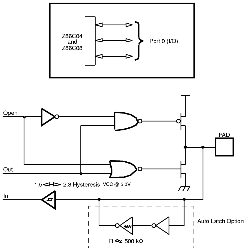
Figure 6. Port 0 Configuration
