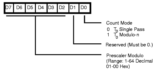
R245 PRE0
