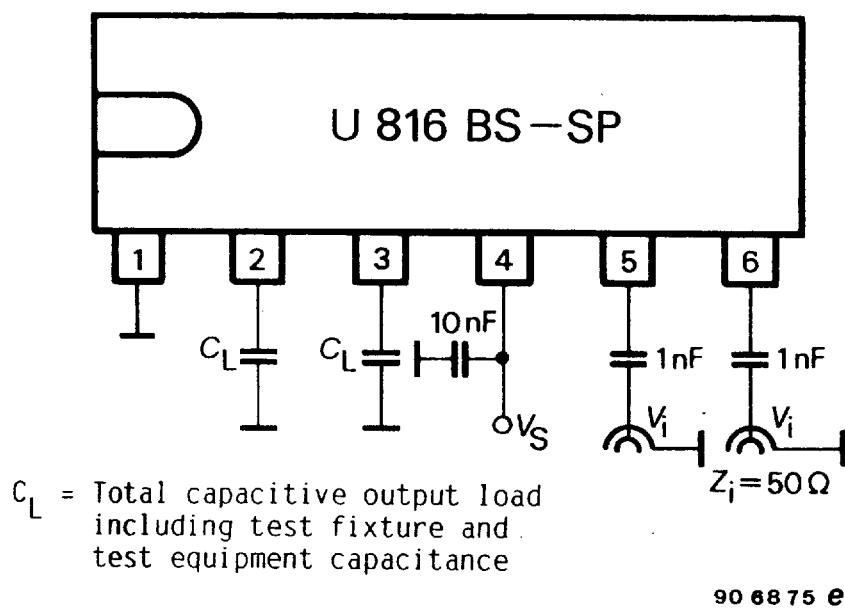
Figure 2. Test circuit
