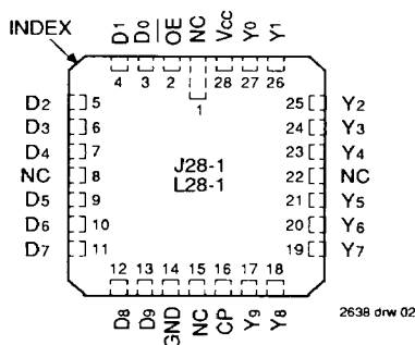
LCC/PLCC TOP VIEW
