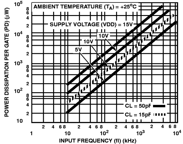
FIGURE 2. TYPICAL POWER DISSIPATION CHARACTERISTICS
