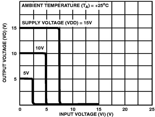
FIGURE 1. TYPICAL VOLTAGE TRANSFER CHARACTERISTICS
