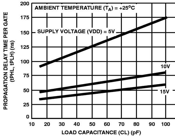
FIGURE 7. TYPICAL PROPAGATION DELAY TIME PER GATE AS A FUNCTION OF LOAD CAPACITANCE
