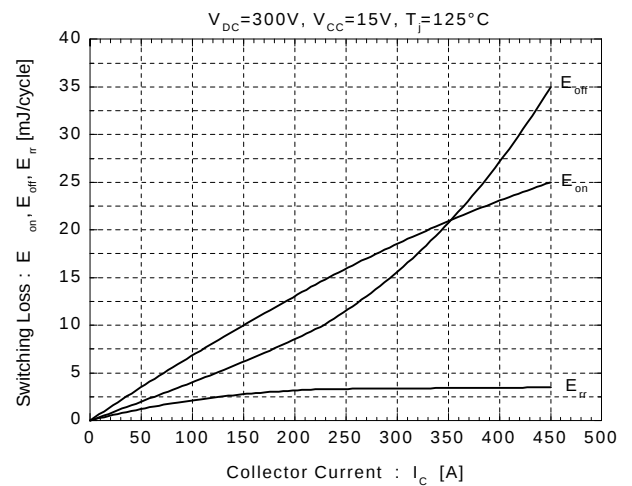
Switching Loss vs. Collector Current
