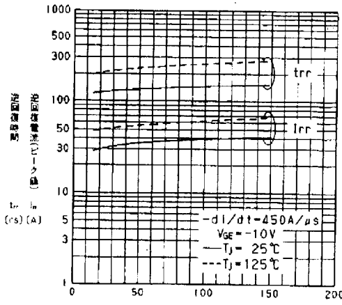
T_{rr}, I_{rr}-I_r 特性 T_{rr}, I_{rr}-I_r
