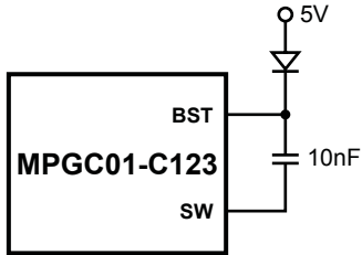
Figure 3—External Bootstrap Diode
