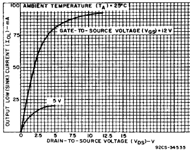
Fig. 3 - Typical N-Channel output low (sink) current characteristics - CMOS to TTL.
