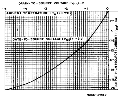
Fig. 7 - Typical P-channel output high (source) current characteristics - CMOS to TTL.
