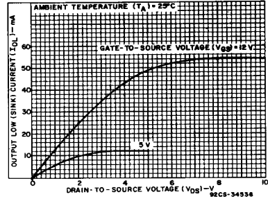
Fig. 4 - Typical output low (sink) current characteristics - TTL to CMOS.
