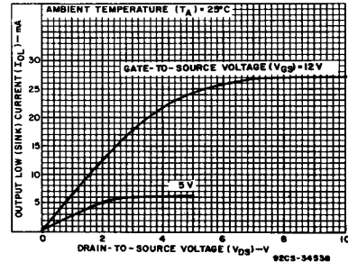
Fig. 6 - Minimum output low (sink) current characteristics - TTL to CMOS.
