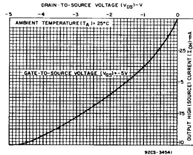
Fig. 9 - Minimum P-Channel output high (source) current characteristic - CMOS to TTL.
