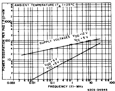
Fig. 13 - Power dissipation as a function of frequency - CMOS to TTL.
