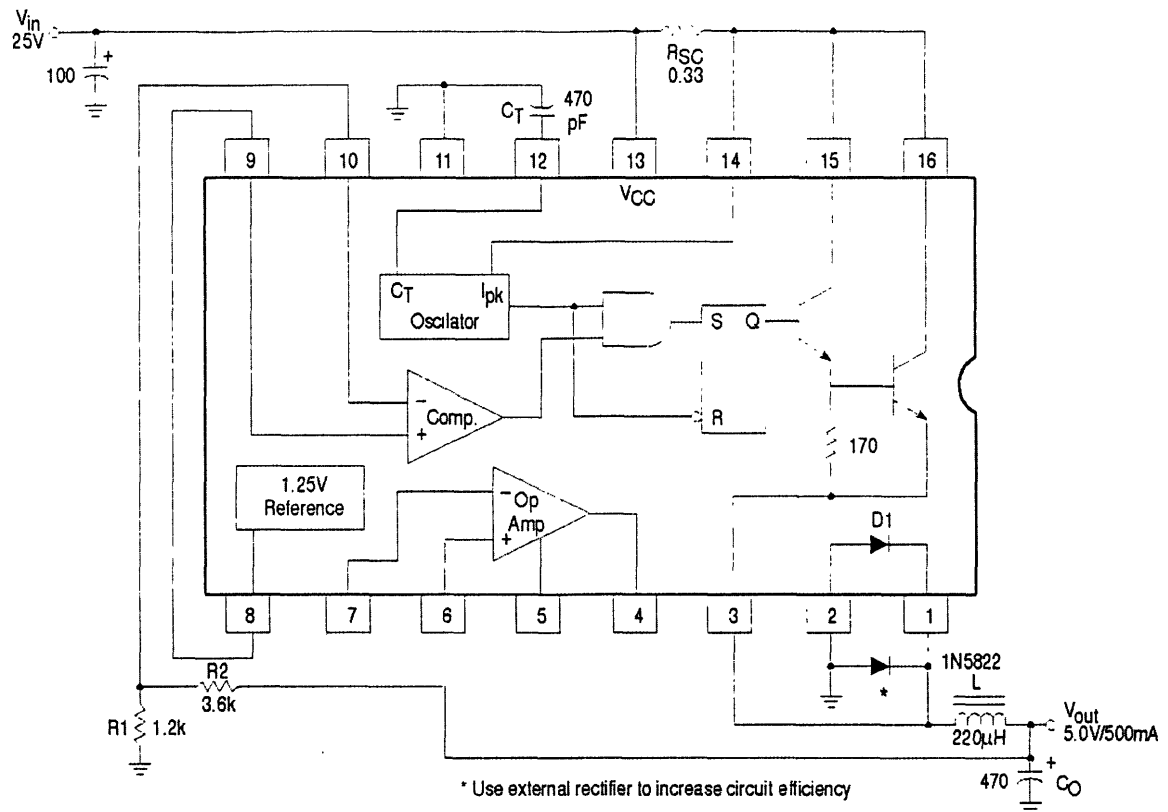
Figure 5. Step-Down Converter
