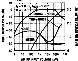
AM Characteristics V_{CC} = 6V
