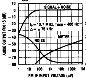
FM IF Characteristics V_{CC} = 6V
