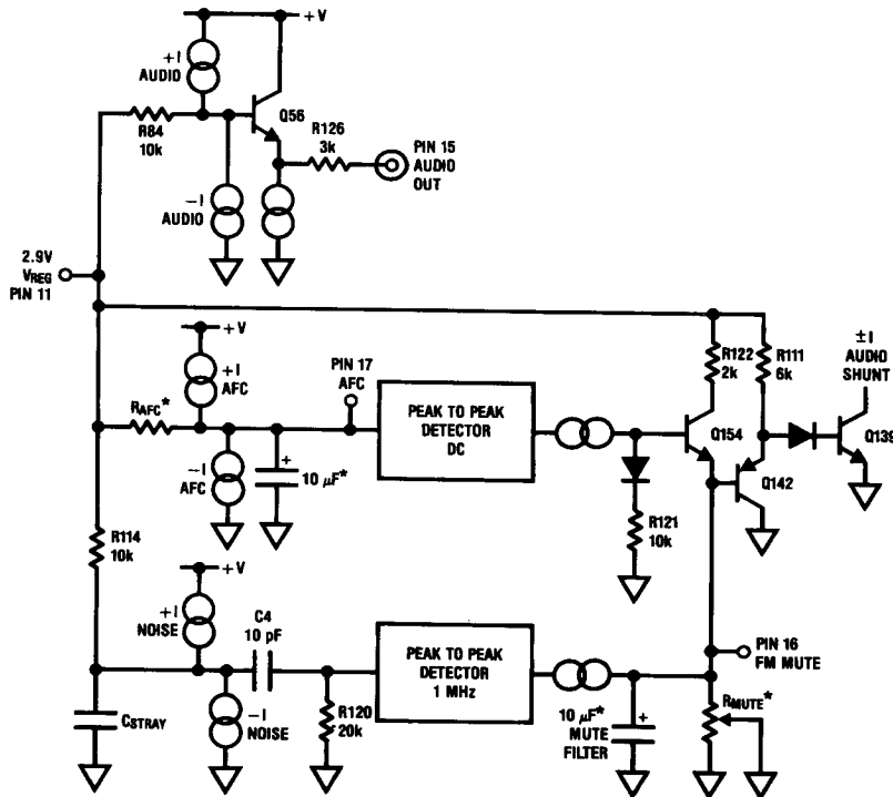
FIGURE 1. Simplified Mute Circuit Schematic
