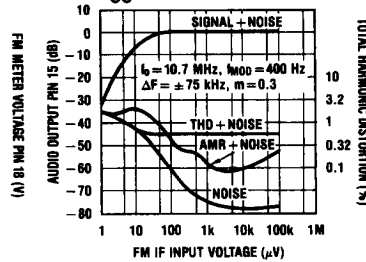
FM IF Characteristics V_{CC} = 6V
