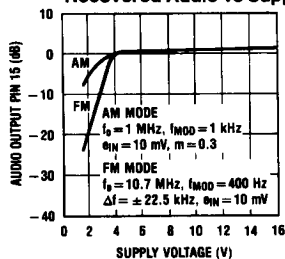
Recovered Audio vs Supply
