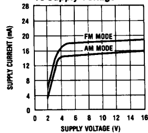
Quiescent Supply Current vs Supply Voltage
