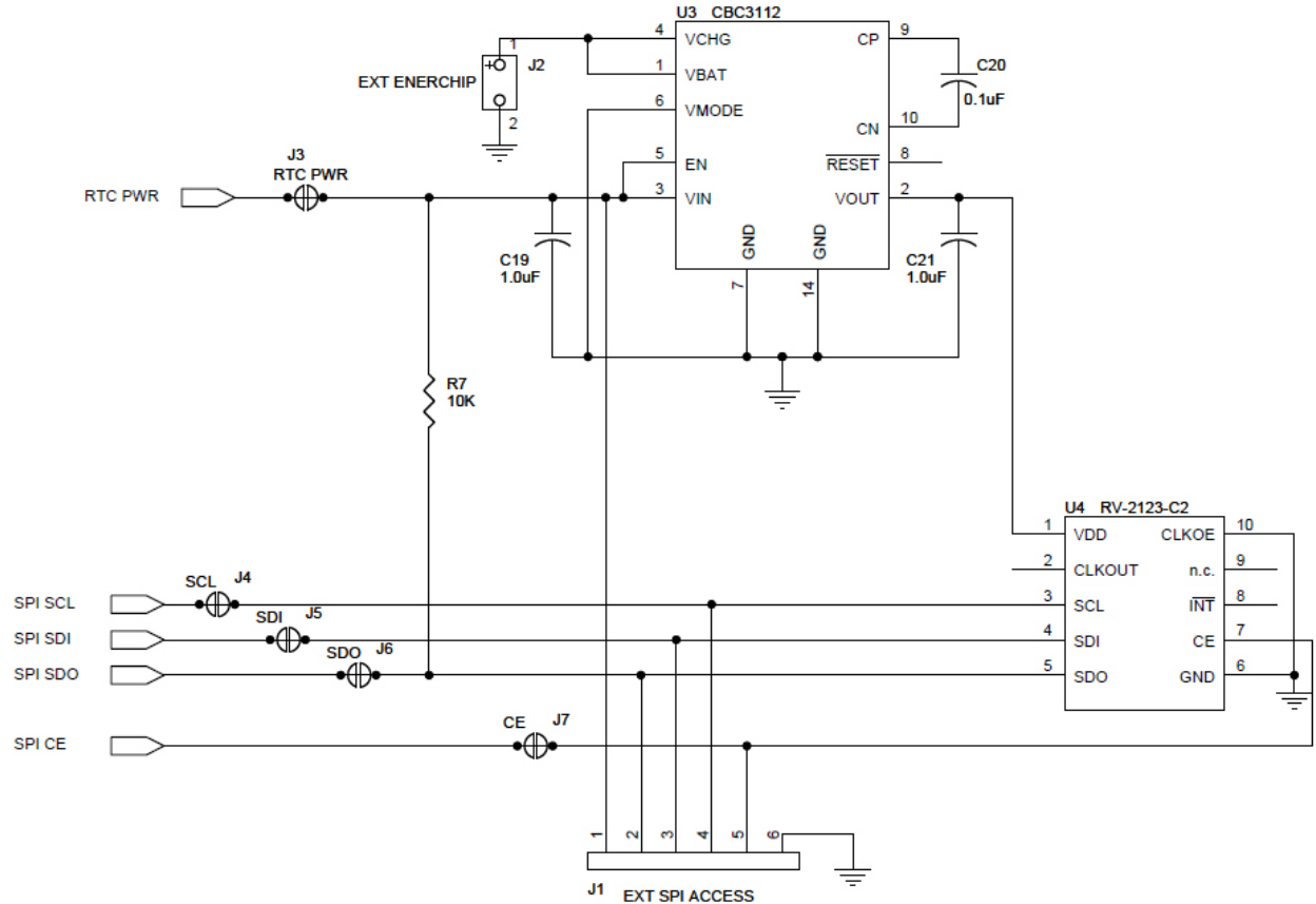
Figure 4: CBC-EVAL-06 Circuit Schematic (EnerChip CC and RTC Portion Only).
