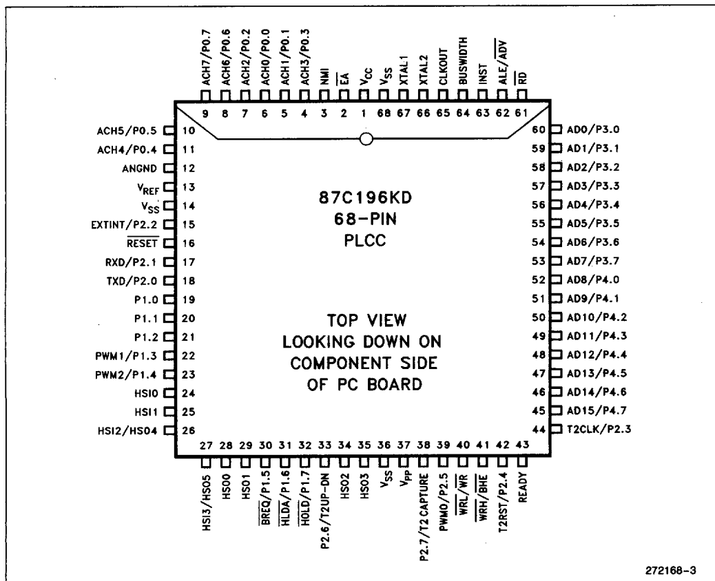
Figure 4. 68-Pin PLCC Package
