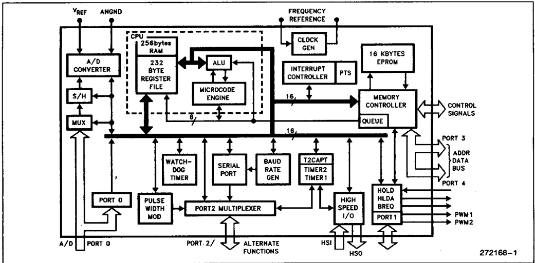
Figure 1. 87C196KD Block Diagram
