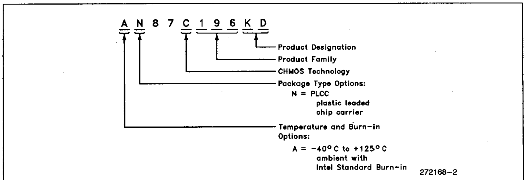
Figure 2. The 87C196KD Family Nomenclature
