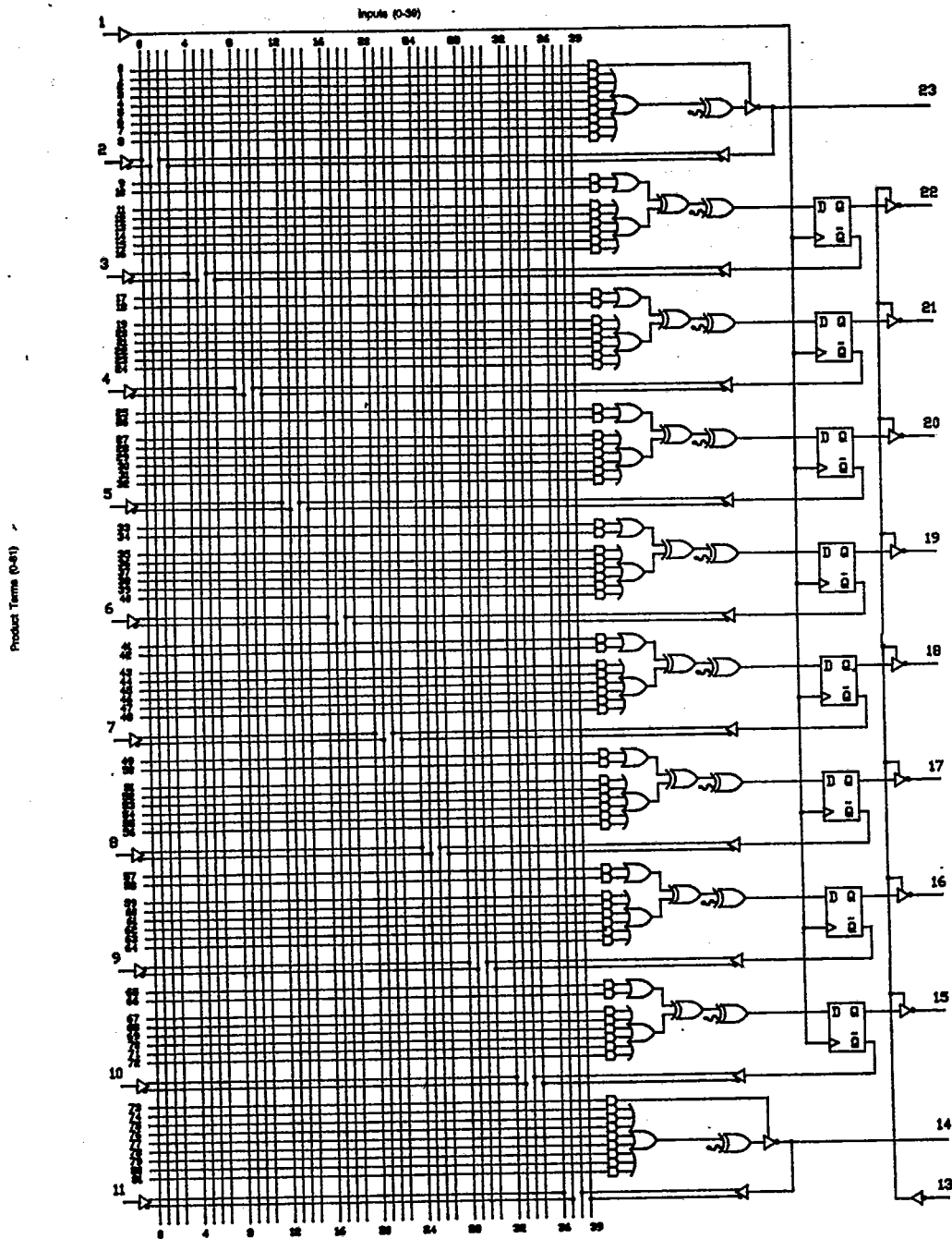
Figure 4. AmPAL20XRP8 Logic Diagram
